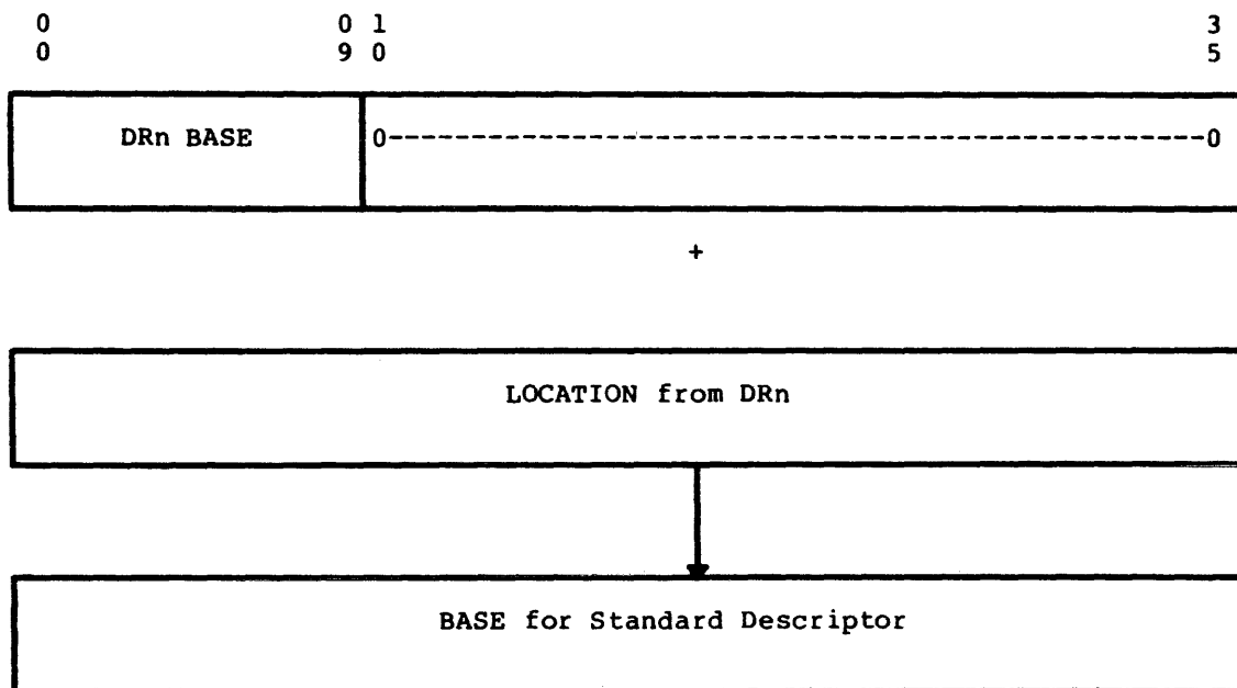
Figure 5-5. BASE For Standard Descriptor (DPS 88)
