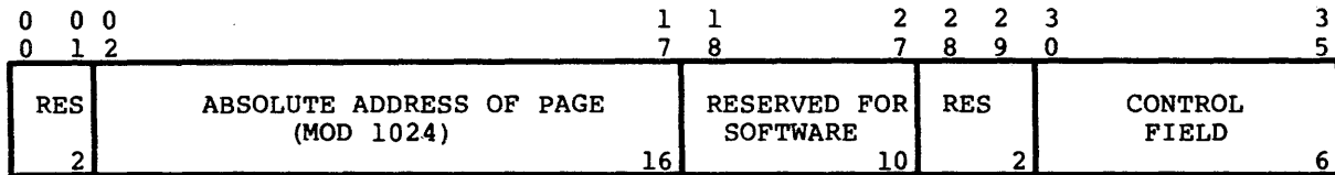
Figure 5-9. Page Table Word Format
