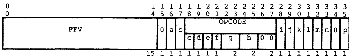
Figure 4-13. Mode Register (MR) Format
