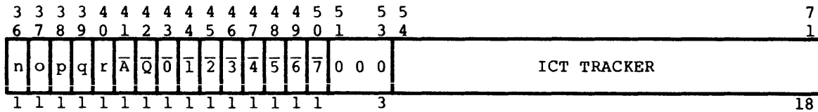
Figure 4-17. Operations Unit History Register (OU n ) Format
