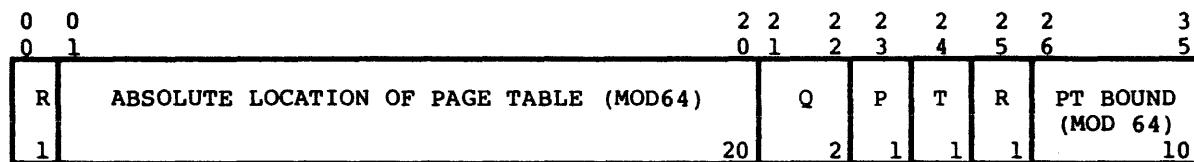
Figure 5-8. Working Space Page Table Directory Format
