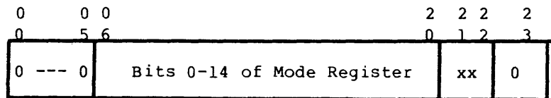
Figure 8-1. Fault Trap Address
