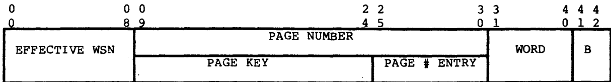
Figure 5-16. Virtual Address, Fragmented Page Table
