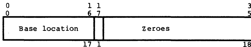
Figure 4-29. Page Directory Base Register (PDBR) Format.
