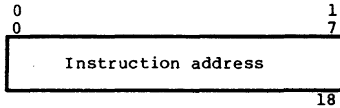
Figure 4-9. Instruction Counter (IC) Format
