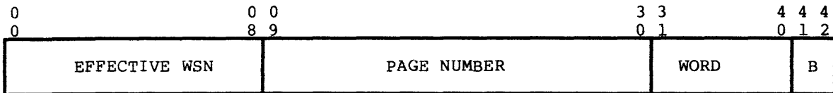
Figure 5-10. Virtual Address
