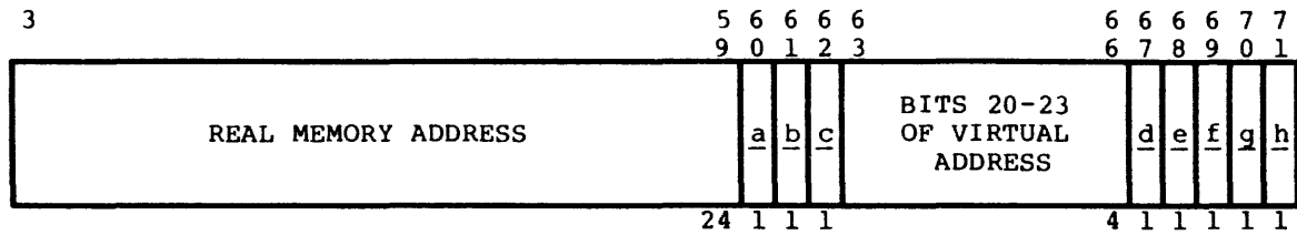
Figure 4-18. Virtual Unit History Register (VUn) Format
