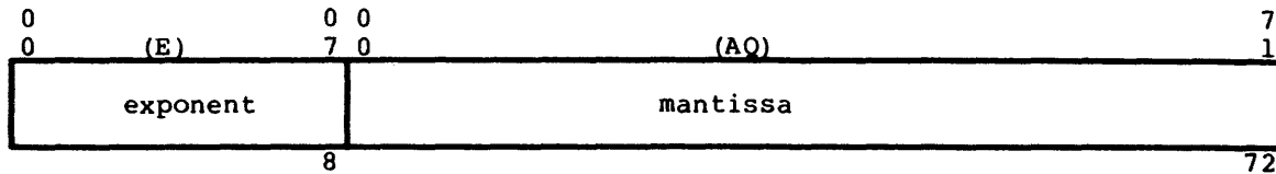
Figure 4-5. Exponent-Accumulator-Quotient Register (EAQ) Format
