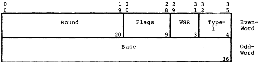
Figure 4-23. Parameter Stack Register (PSR) Format
