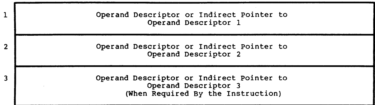
Figure 7-2. Multiword Instruction Format
