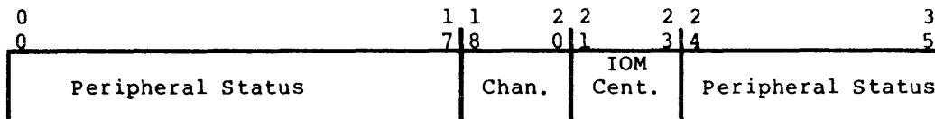
Figure 8-2. Channel Status Word
