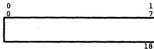
Figure 4-6. Index Register (Xn) Format
