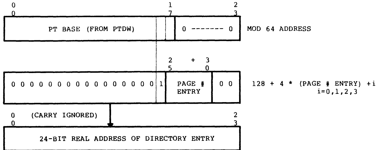
Figure 5-18. Fragmented Page Table Addressing (DPS 8)
