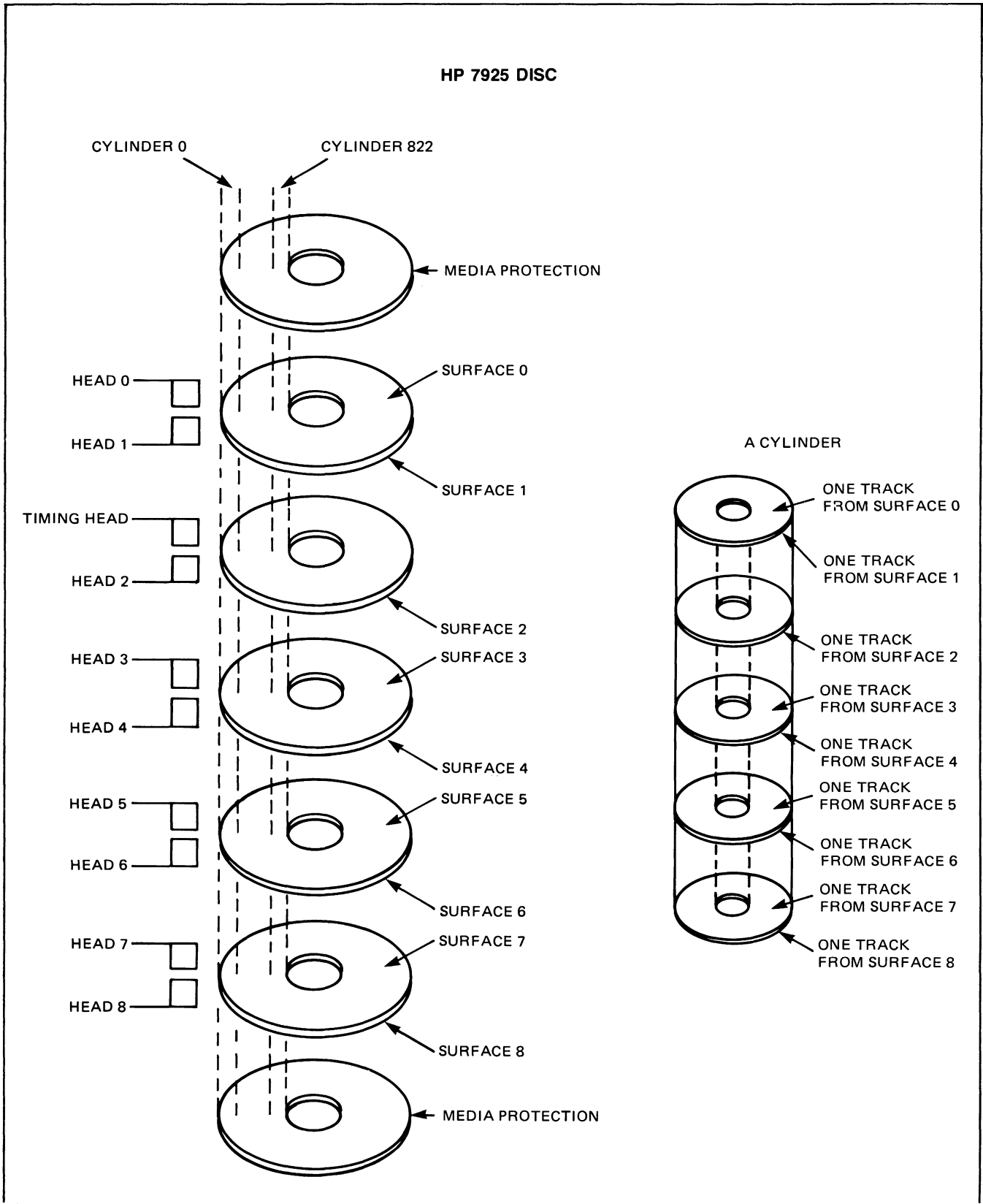
Figure 3-7. HP 7925 Disc
