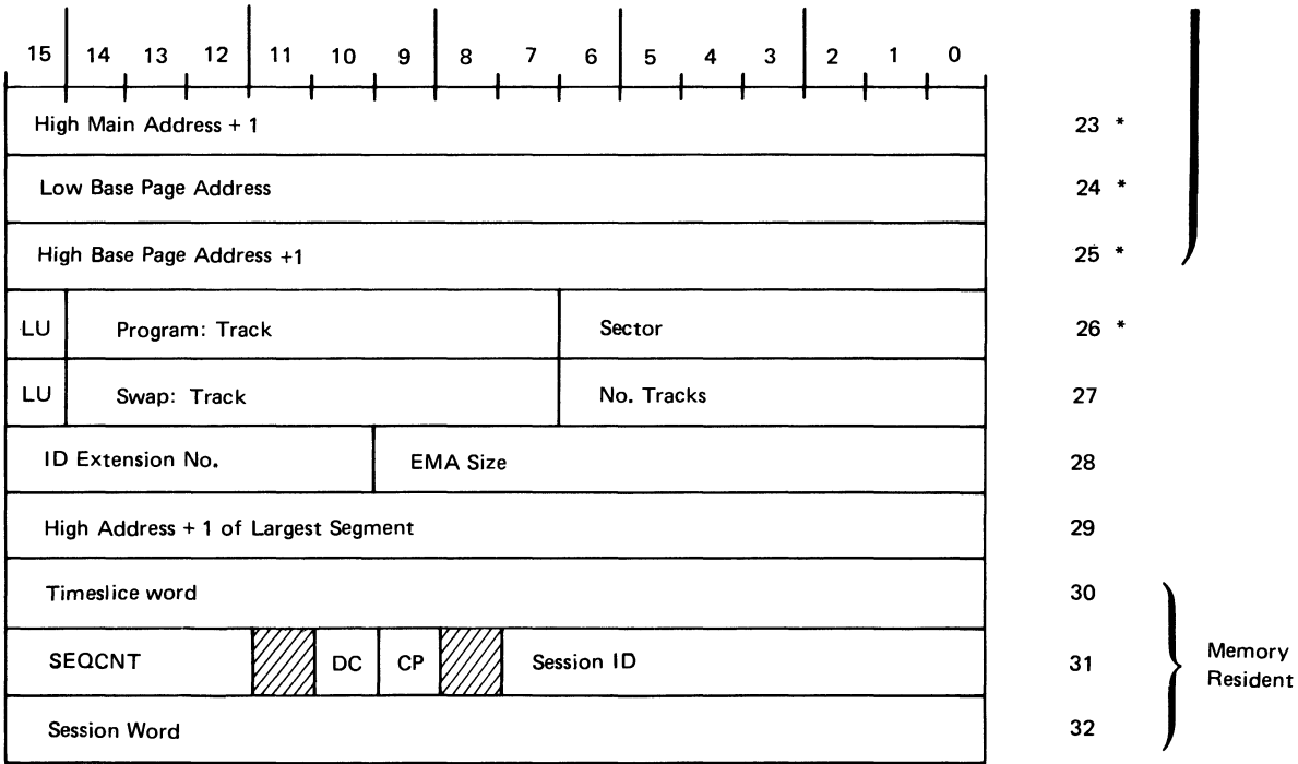
Figure C-1. ID Segment Format (Continued)
