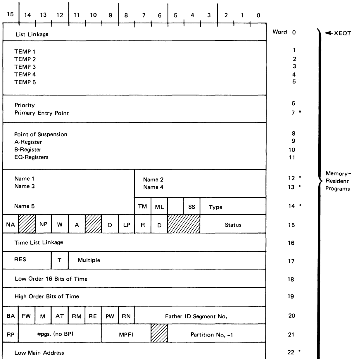
Figure C-1. ID Segment Format
