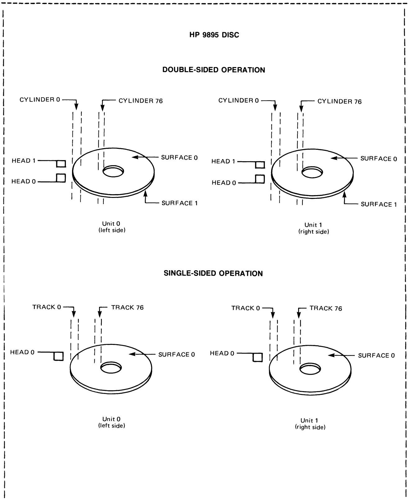
Figure 3-9. HP 9895 Disc.
