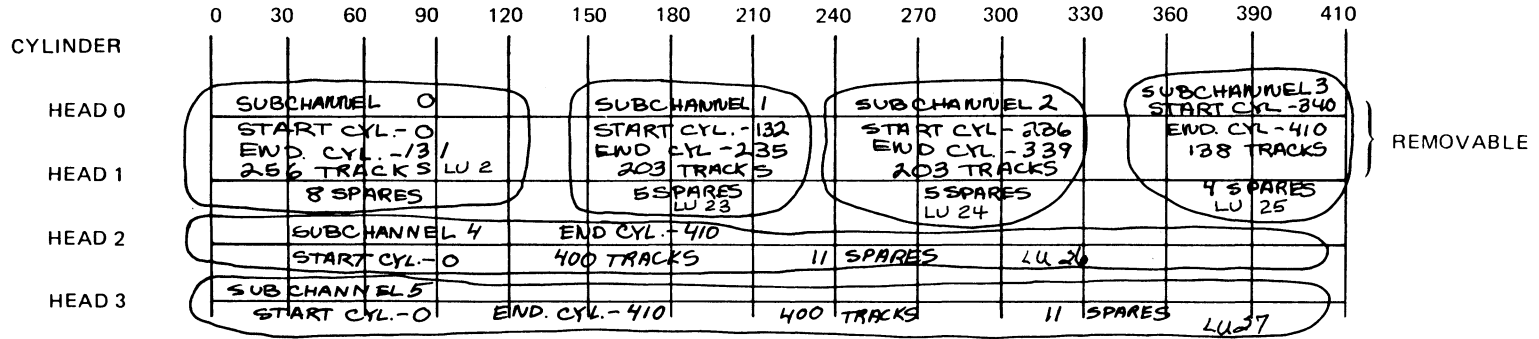
Figure 3-5. HP 7906 Disc Worksheet Example
