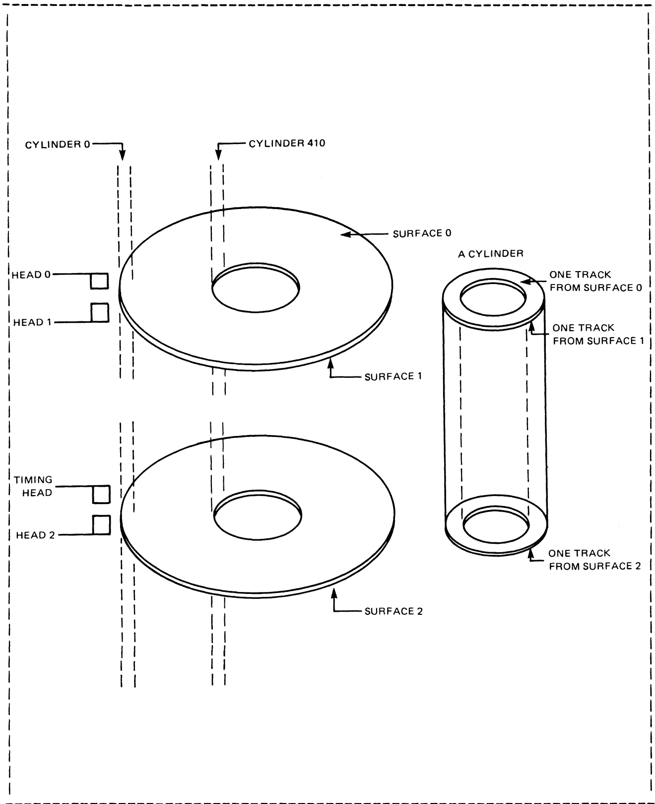
Figure 3-2. HP 7905 Disc
