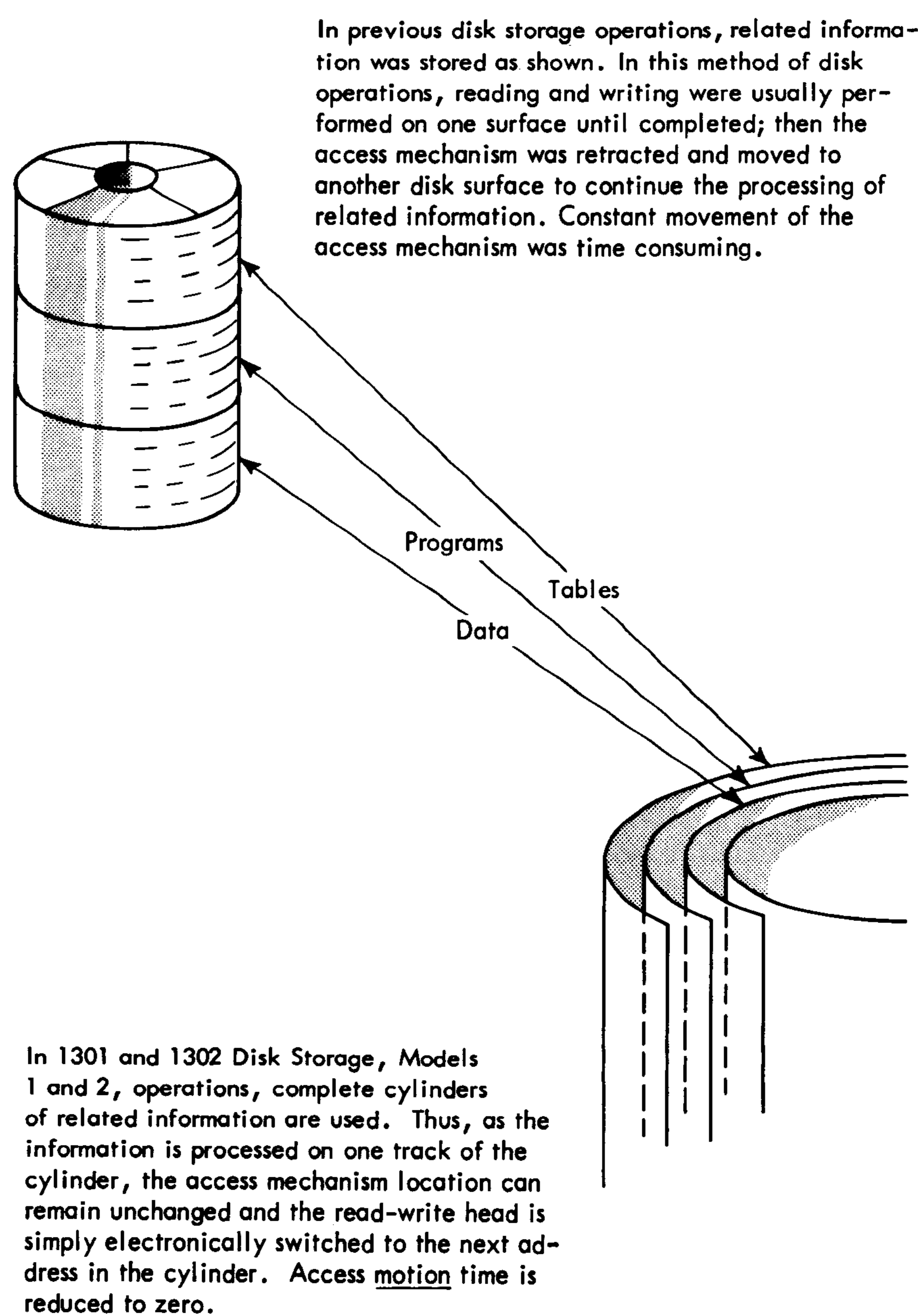
Figure 3. Disk Storage Cylinder Operation
