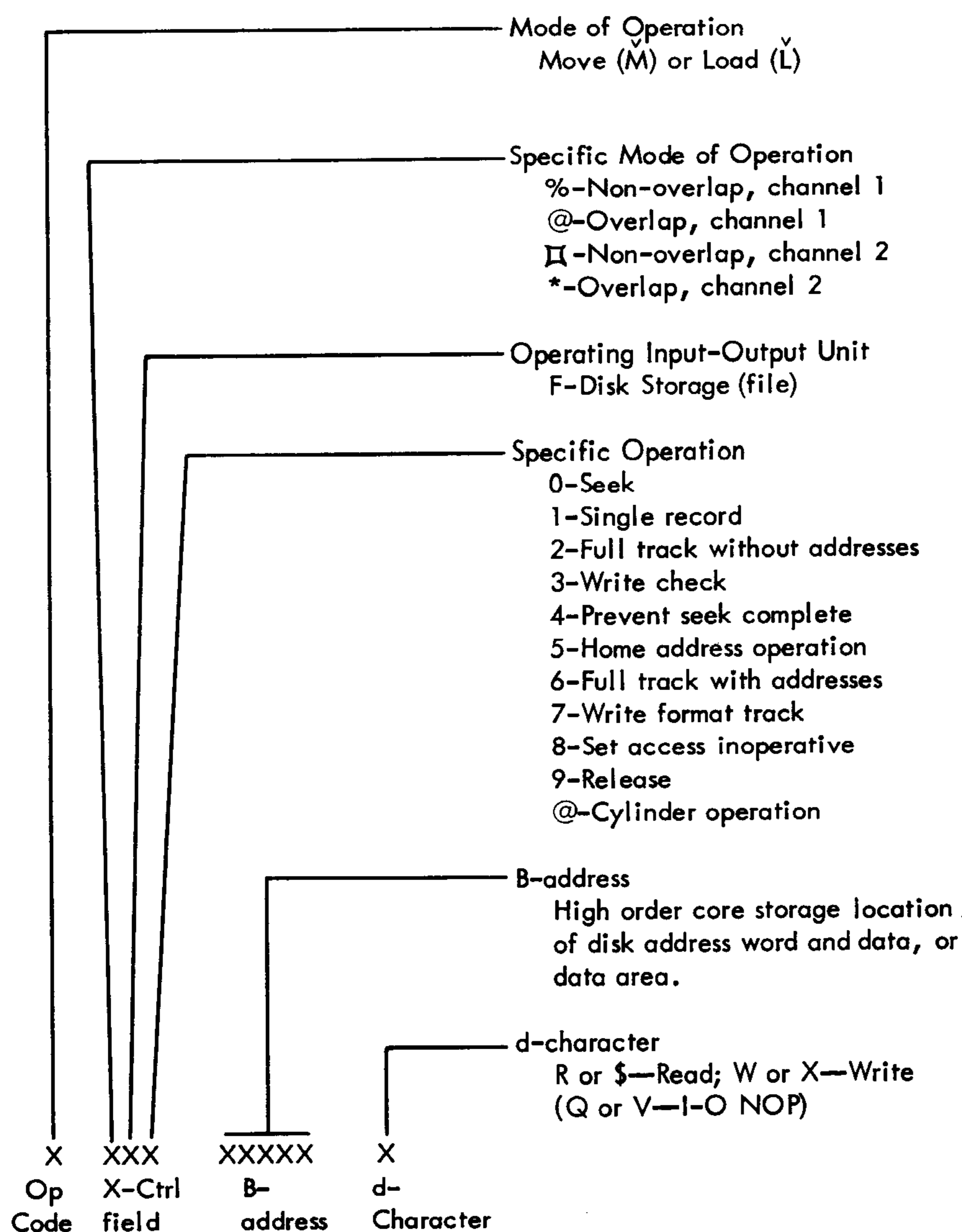
Figure 10. Disk Storage Operation Code Format
