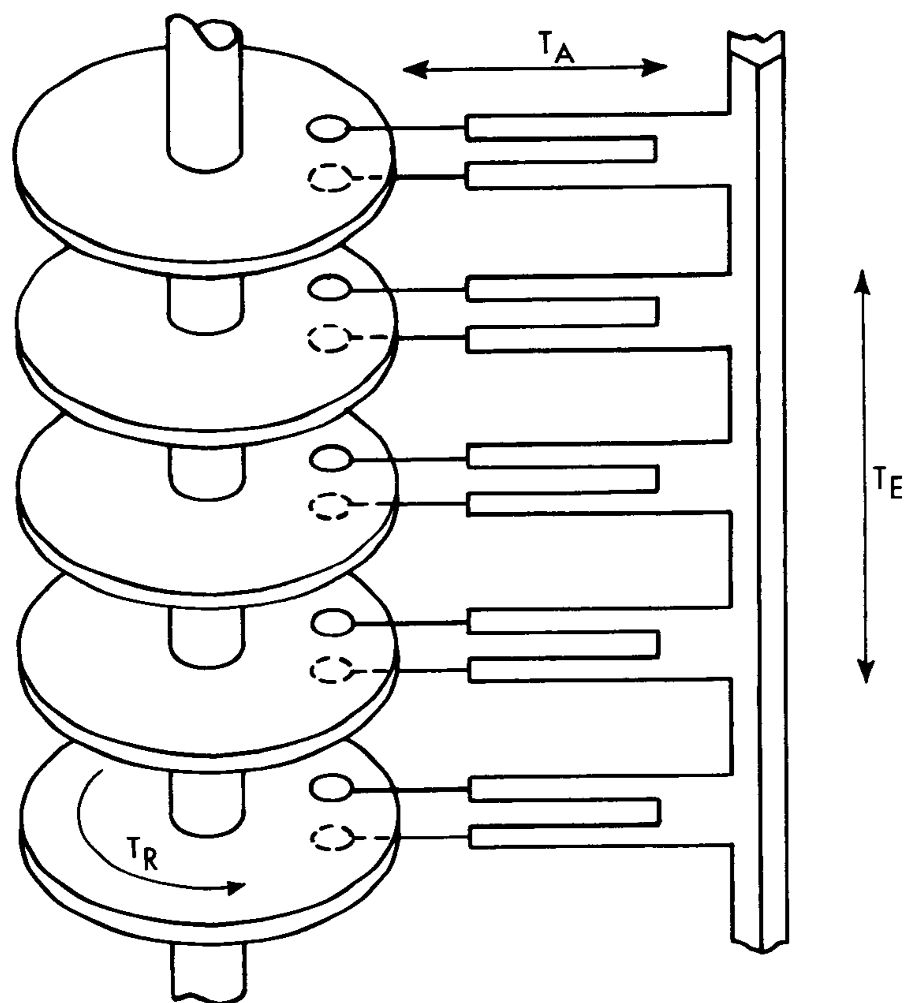
Figure 4. Disk Access Time Requirements
