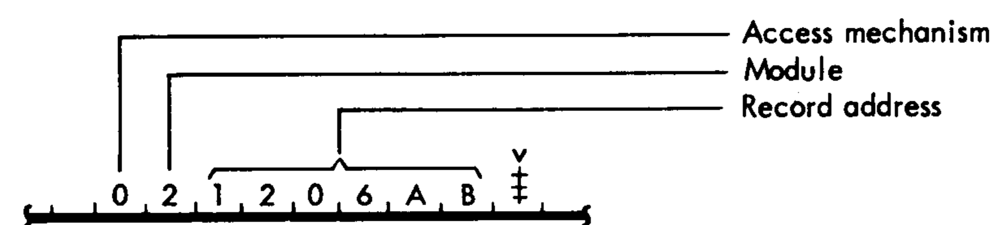
Figure 20. Disk Control Word – Write Single Record
