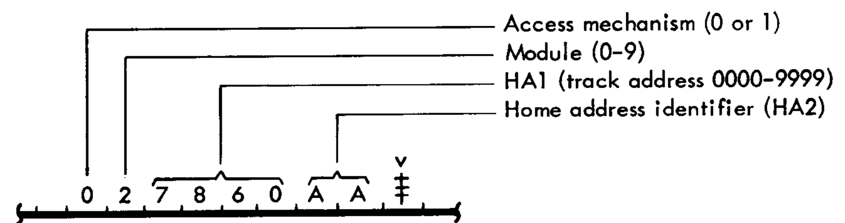
Figure 11. Core Storage Disk Address Word
