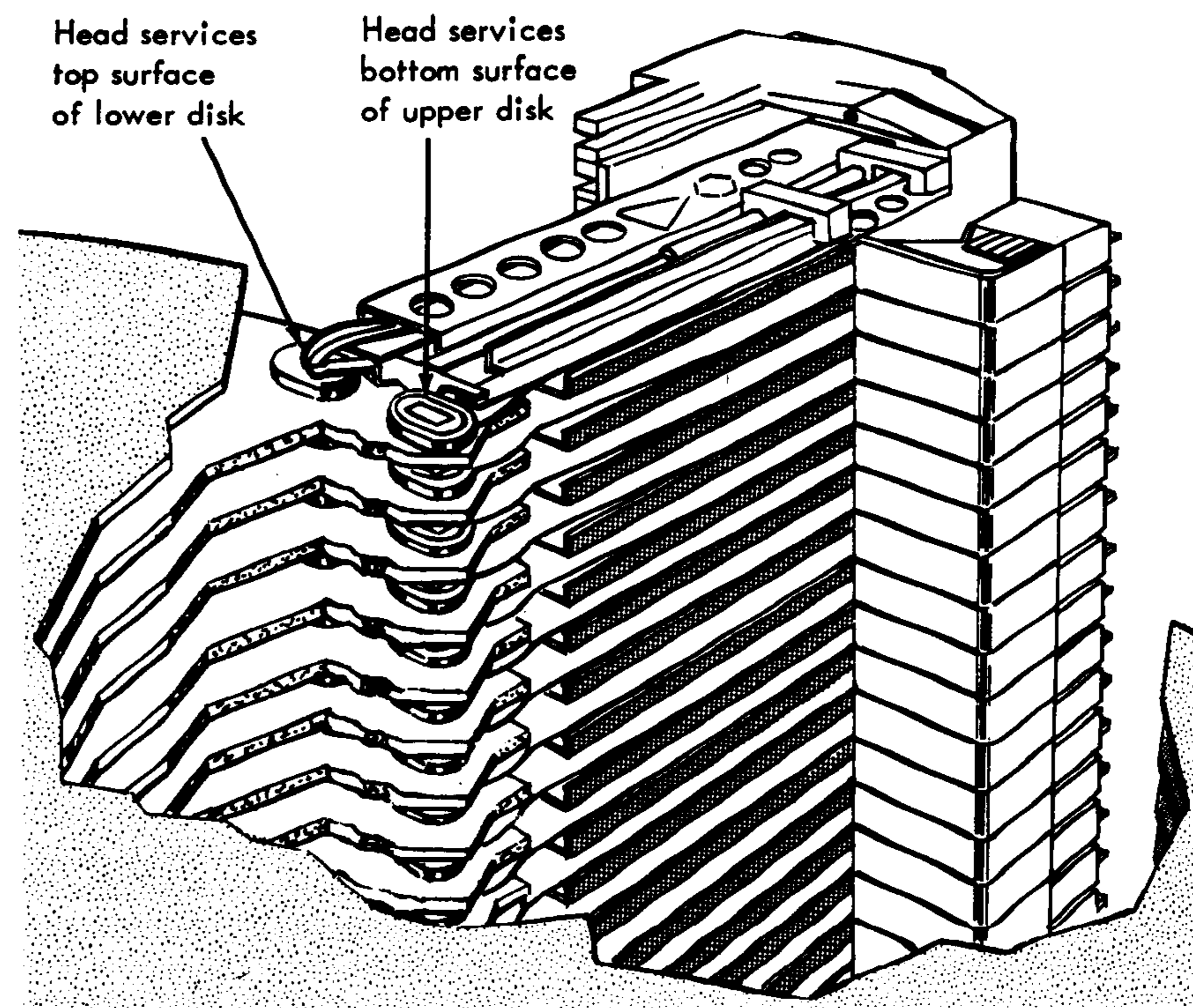
Figure 2. Head Arrangement
