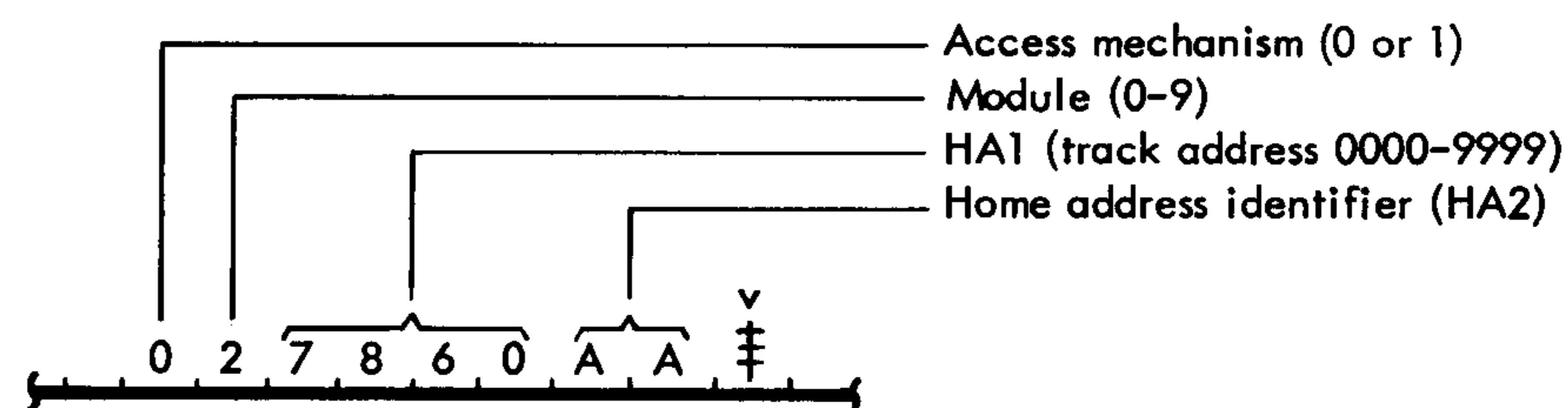
Figure 14. Core Storage Layout – Disk Address Word
