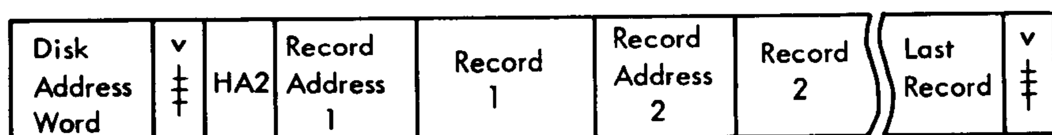
Figure 16. Core Storage Layout – Write/Read Full Track With Home Address
