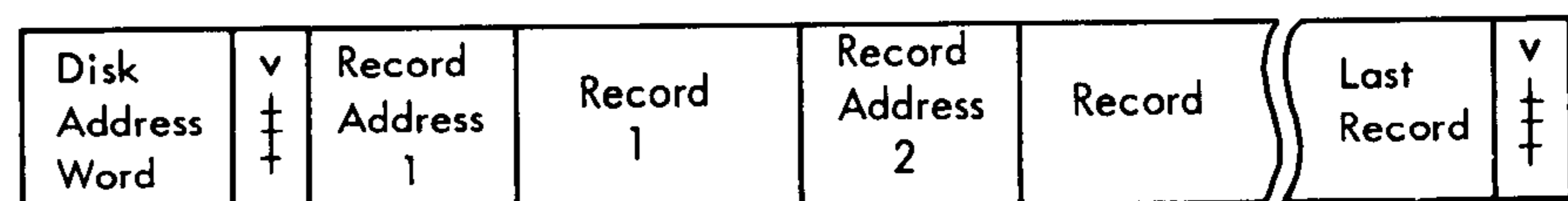
Figure 17. Core Storage Layout – Write/Read Full Track
