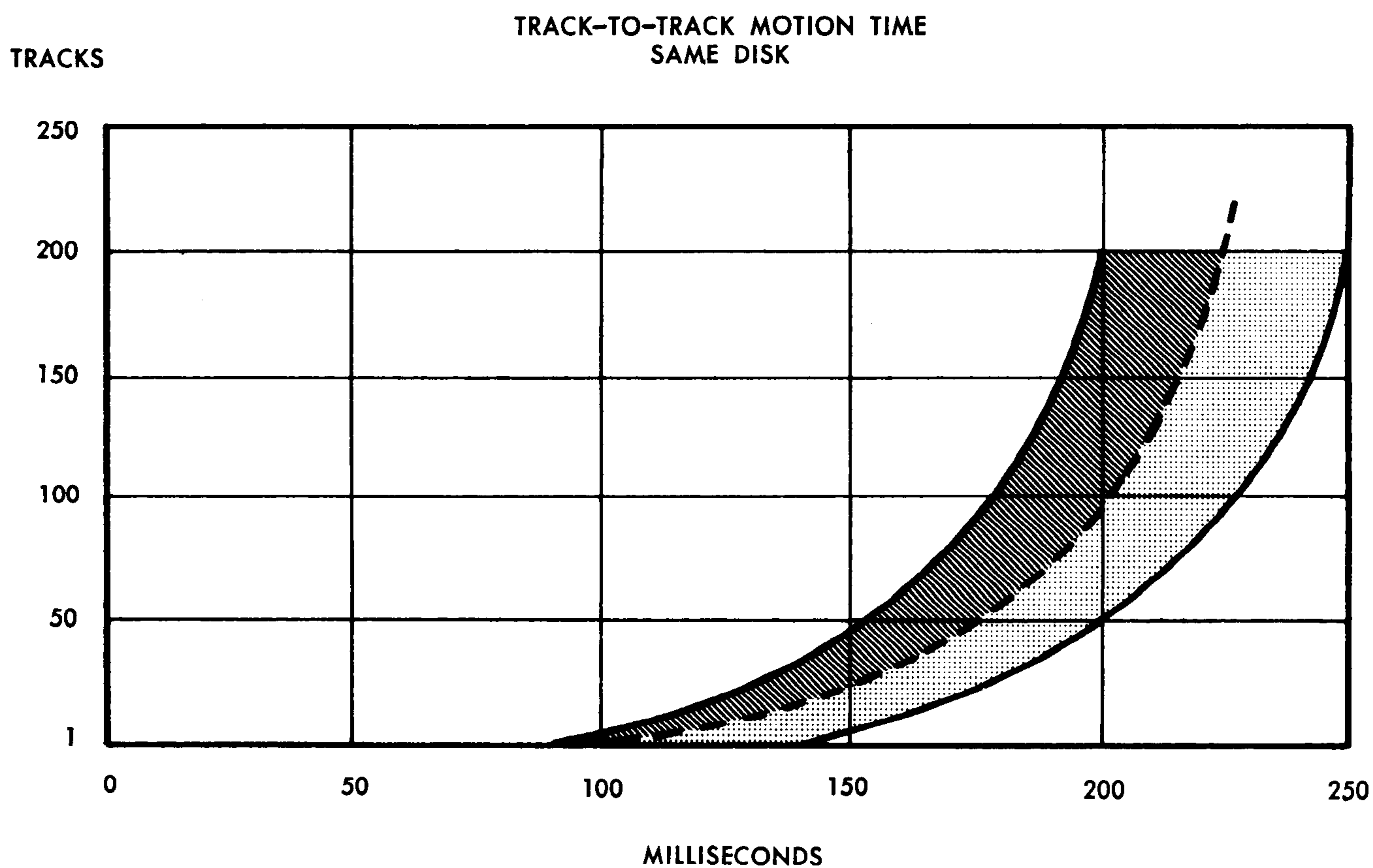
Figure 11. Track-to-Track Motion Time—Same Disks
