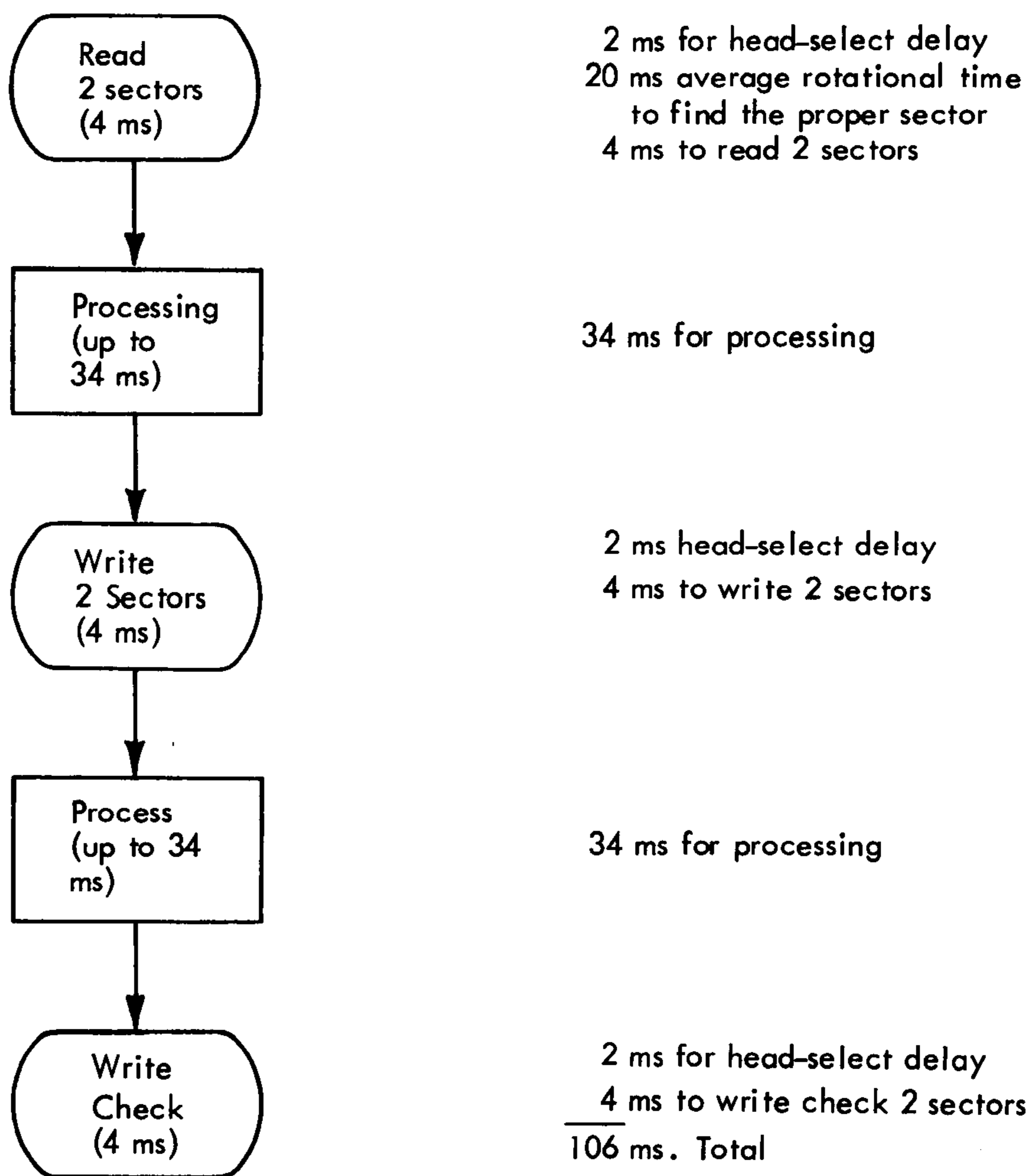
Figure 35. Disk-Storage Timing for a Two-Sector Record
