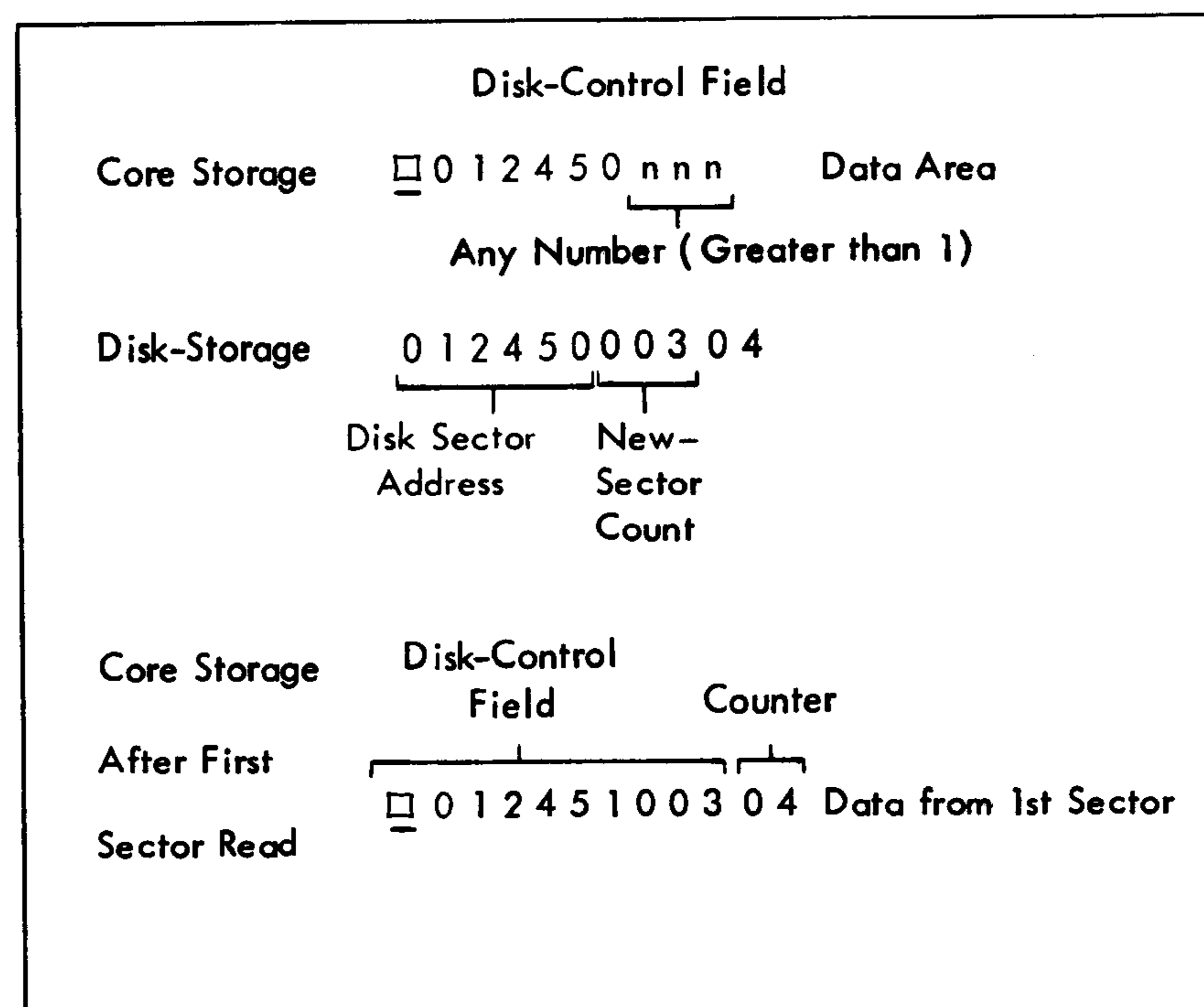
Figure 42. Read Disk—Sector-Count Overlay Operation
