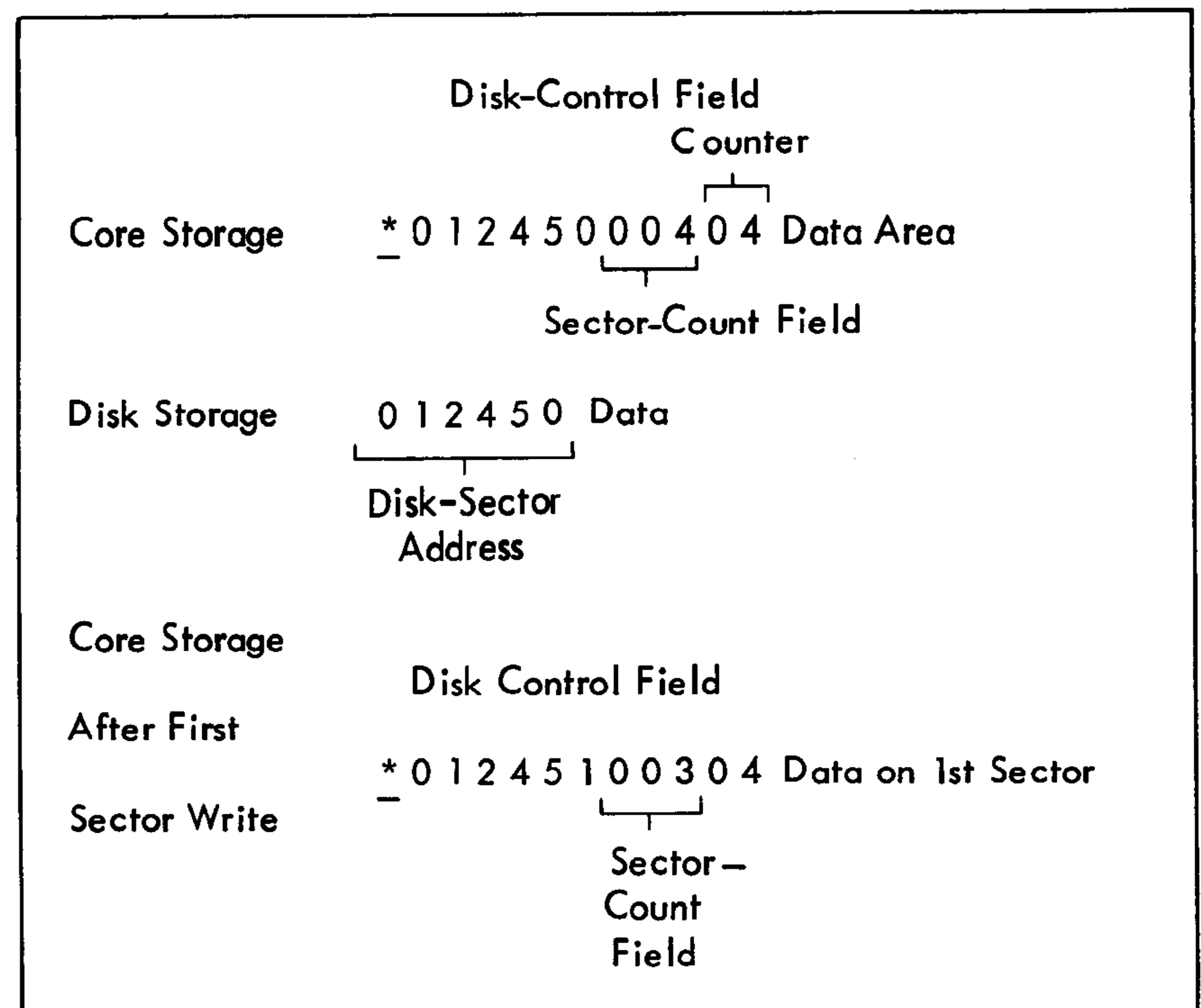
Figure 26. Write Disk—Sector-Count Overlay Operation
