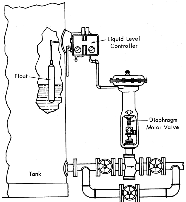
Liquid Level Float
