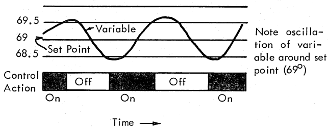
On-Off Control
