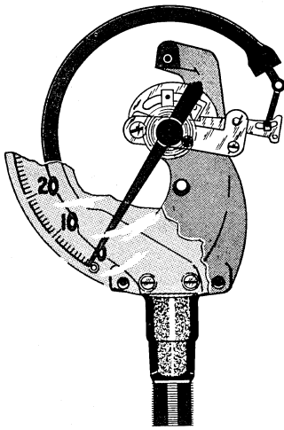
Pressure Gage
