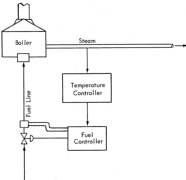
Cascade Control
