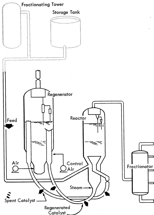
Figure 2. Fluid Catalytic Cracking Process Diagram
