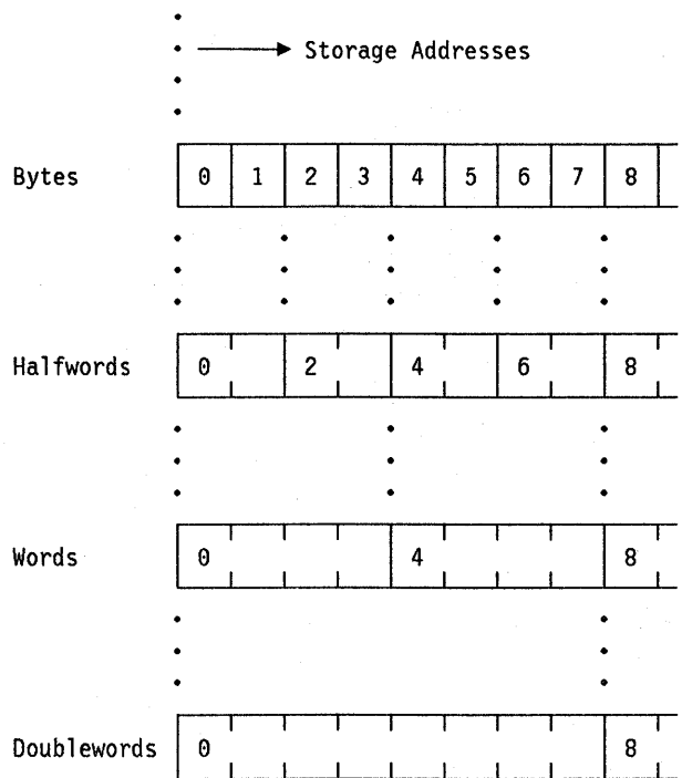
Figure 3-1. Integral Boundaries with Storage Addresses
