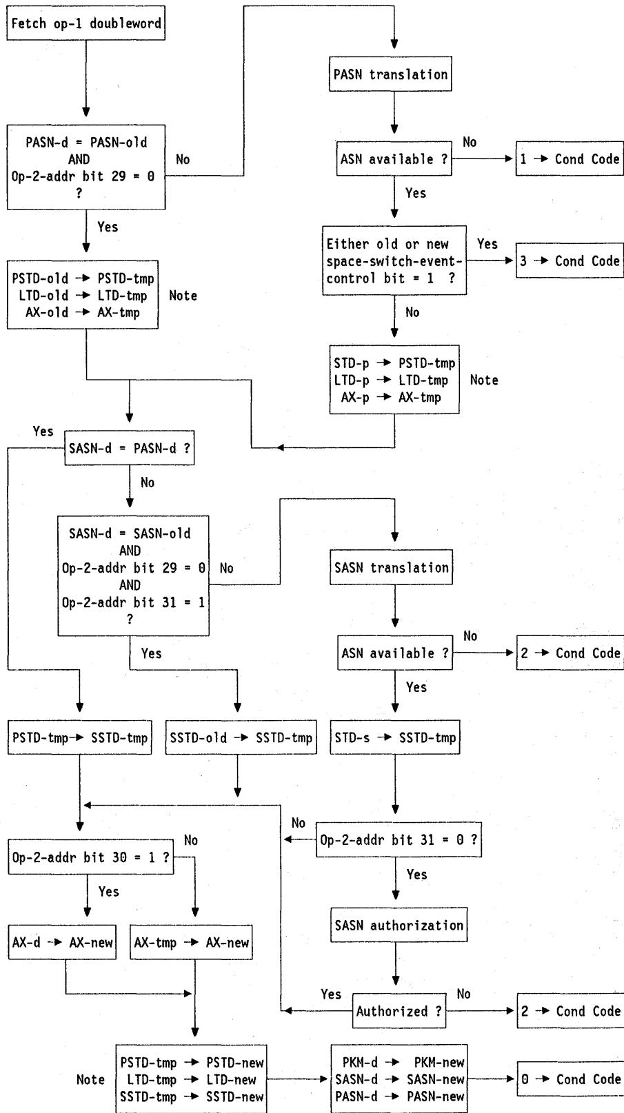
Figure 10-12. Execution of LOAD ADDRESS SPACE PARAMETERS
