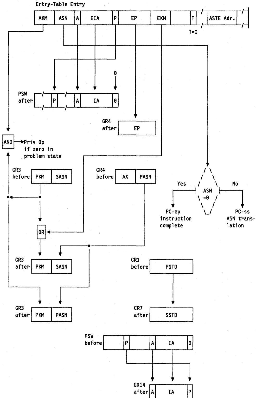
Figure 10-17 (Part 2 of 4). Execution of PROGRAM CALL
