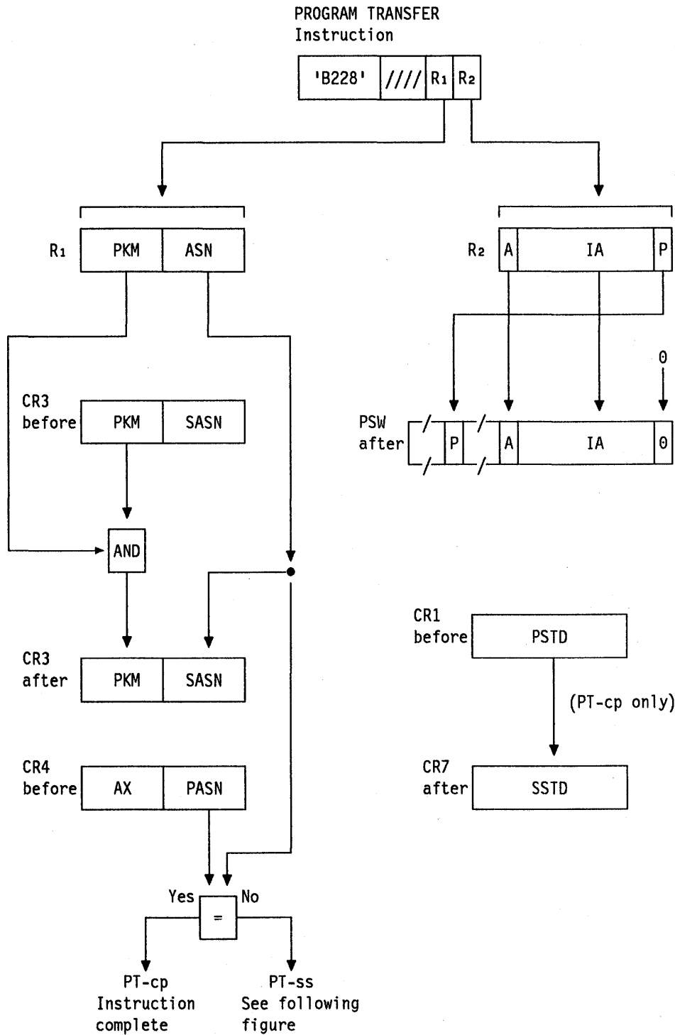
Figure 10-20 (Part 1 of 2). Execution of PROGRAM TRANSFER
