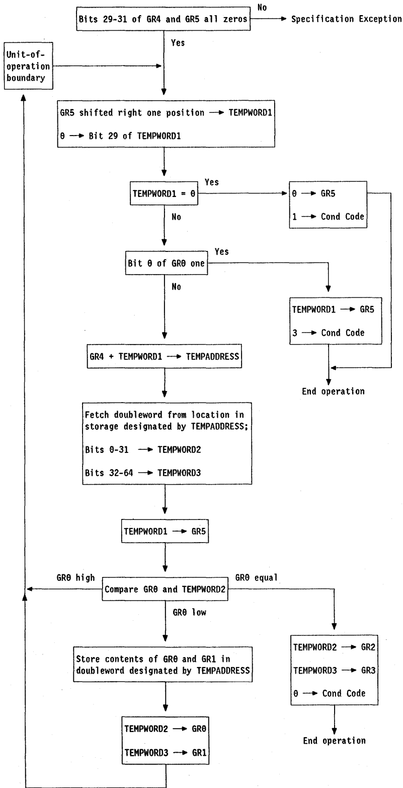
Figure 7-6. Execution of UPDATE TREE
