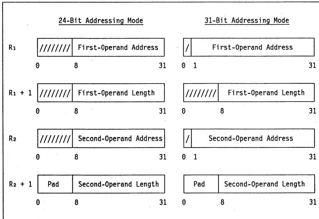
Figure 7-4. Register Contents for COMPARE LOGICAL LONG
