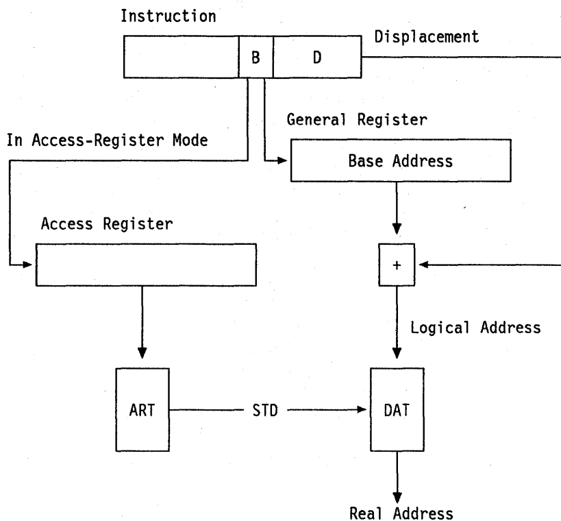
Figure 5-7. Use of Access Registers
