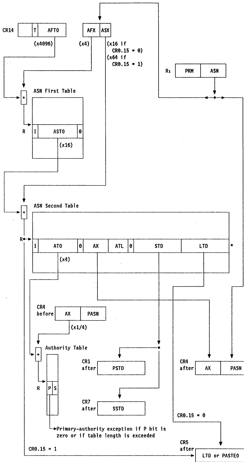
Figure 10-20 (Part 2 of 2). Execution of PROGRAM TRANSFER
