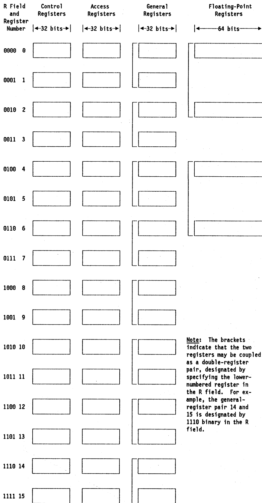
Figure 2-2. Control, Access, General, and Floating-Point Registers
