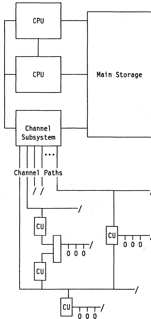
Figure 2-1. Logical Structure of an ESA/370 System with Two CPUs
