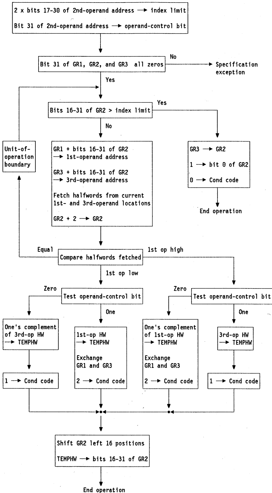
Figure 7-3. Execution of COMPARE AND FORM CODEWORD
