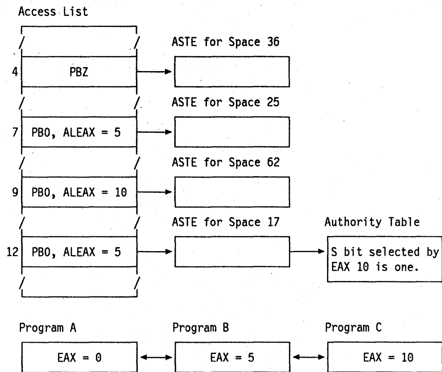
Figure 5-8. Example of Authorizing the Use of Access-List Entries
