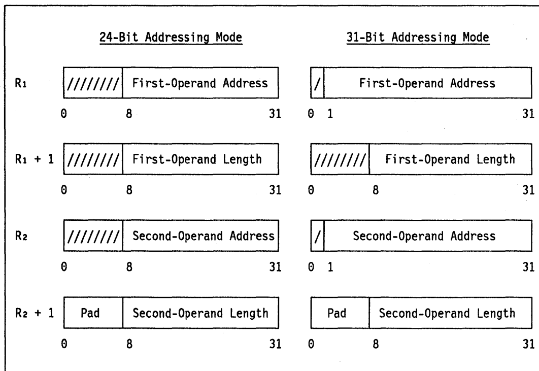
Figure 7-5. Register Contents for MOVE LONG
