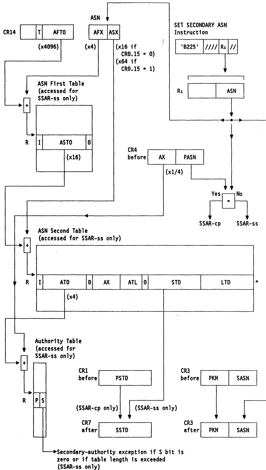
Figure 10-23. Execution of SET SECONDARY ASN
