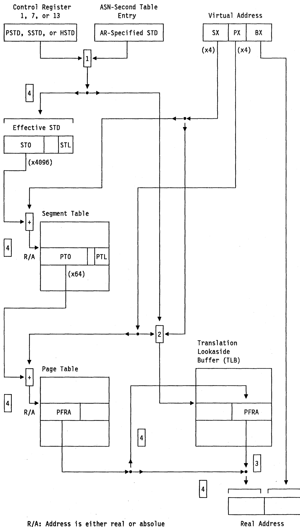
Figure 3-9 (Part 2 of 2). Translation Process
