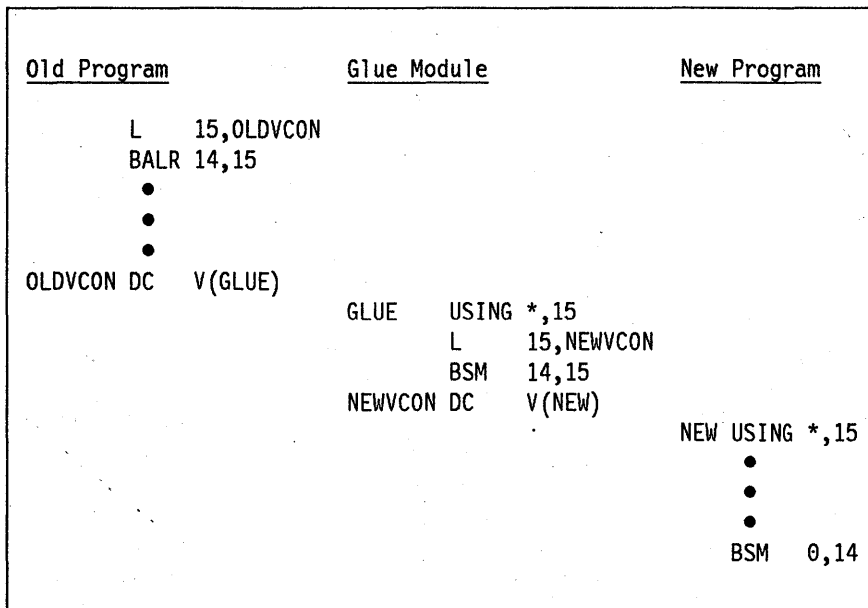
Figure 5-3. Glue Module
