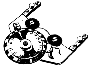
**123635 GAUGE, COUNTER 402-405
