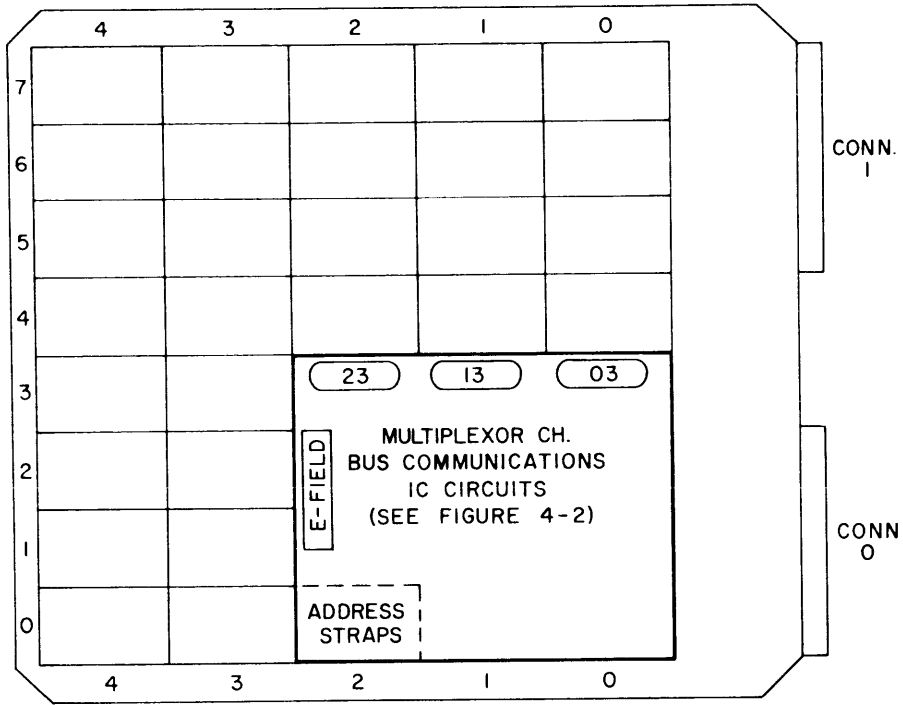
Figure 4-1. Standard I/O Board Layout
