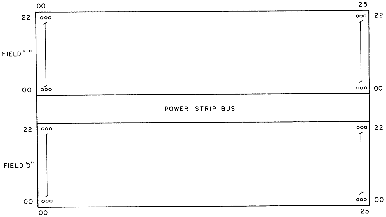
Figure 1-12. Typical INTERDATA Card File, Back Panel Layout
