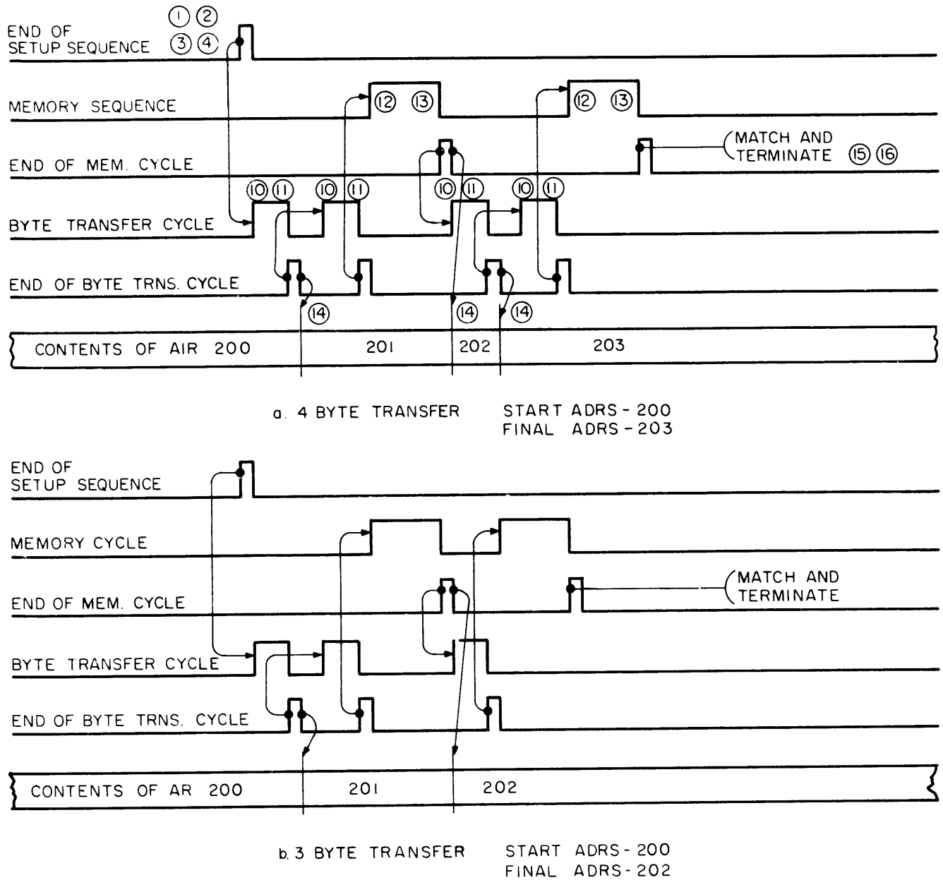
Figure 1-7. Selector Channel Input Operation Timing
