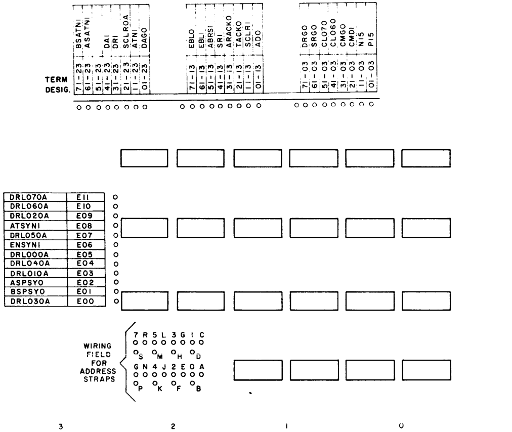
Figure 4-2. Standard I/O Board Field Layout
