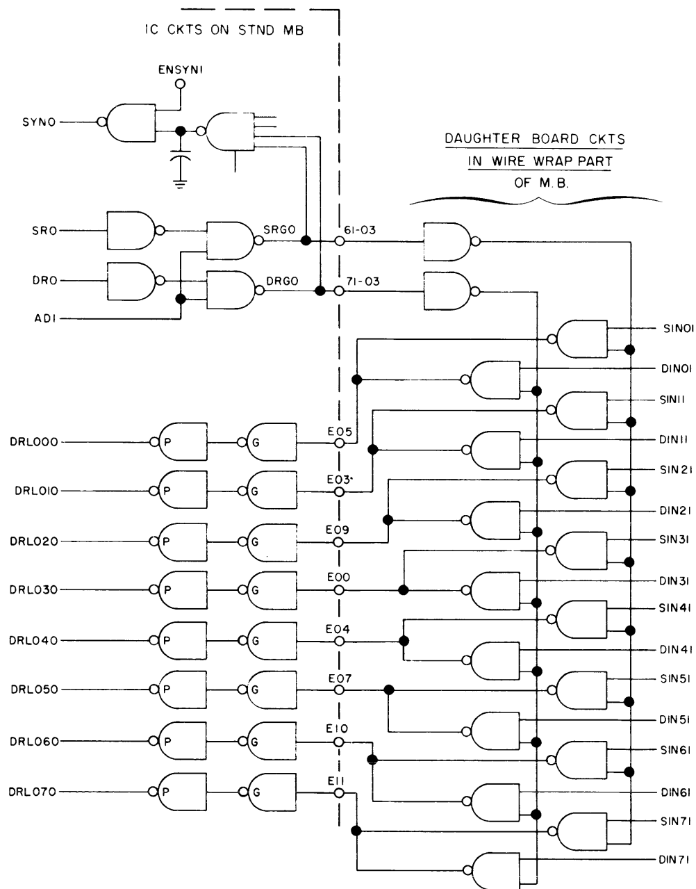
Figure 4-4. Data and Status Request, Logic Diagram
