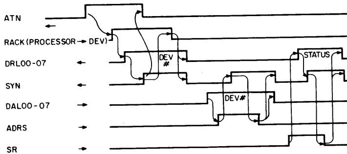
Figure 2-18. Acknowledge Interrupt Instruction Timing
