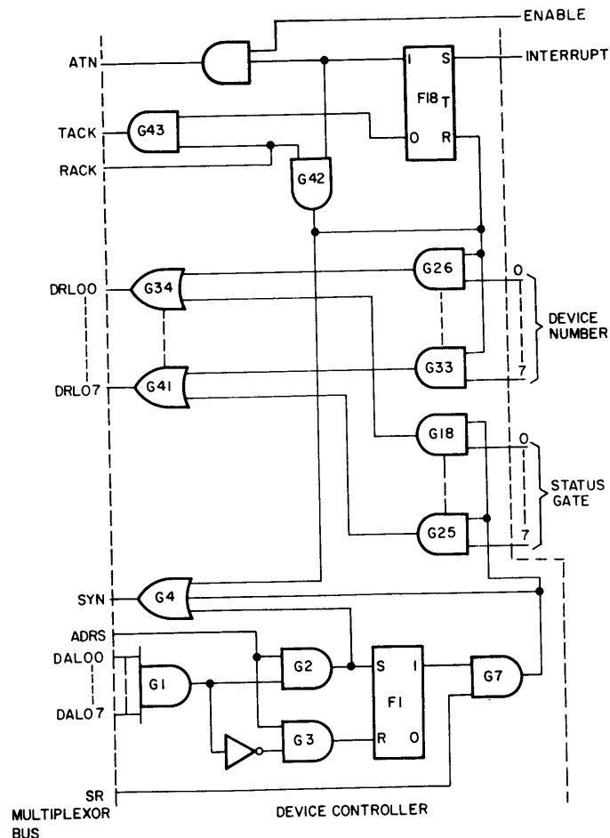
Figure 2-19. Device Controller Logic for Acknowledge Interrupt Instruction
