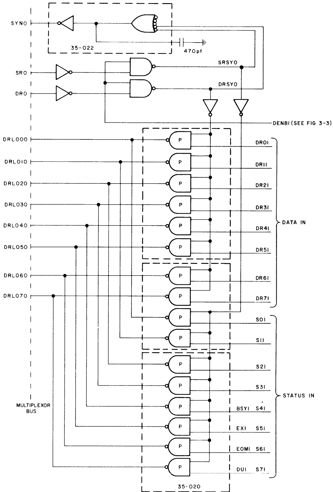
Figure 3-4. Data and Status Input, Logic Diagram
