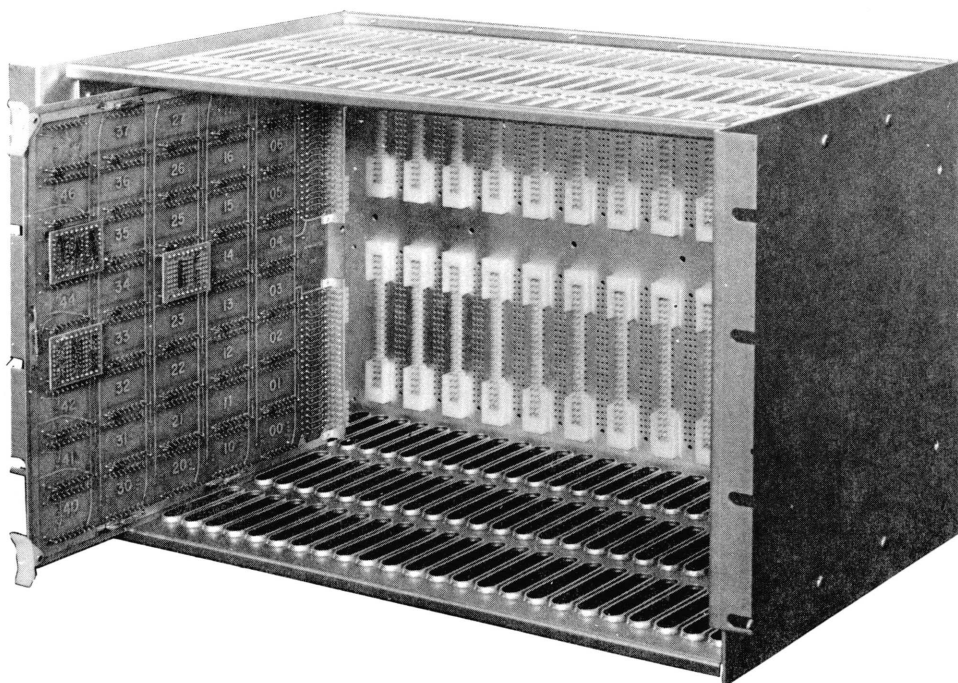
Figure 1-10. Typical INTERDATA Card File, Three Quarter Front View
