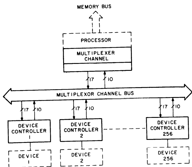
Figure 1-3. Multiplexor Channel, Block Diagram
