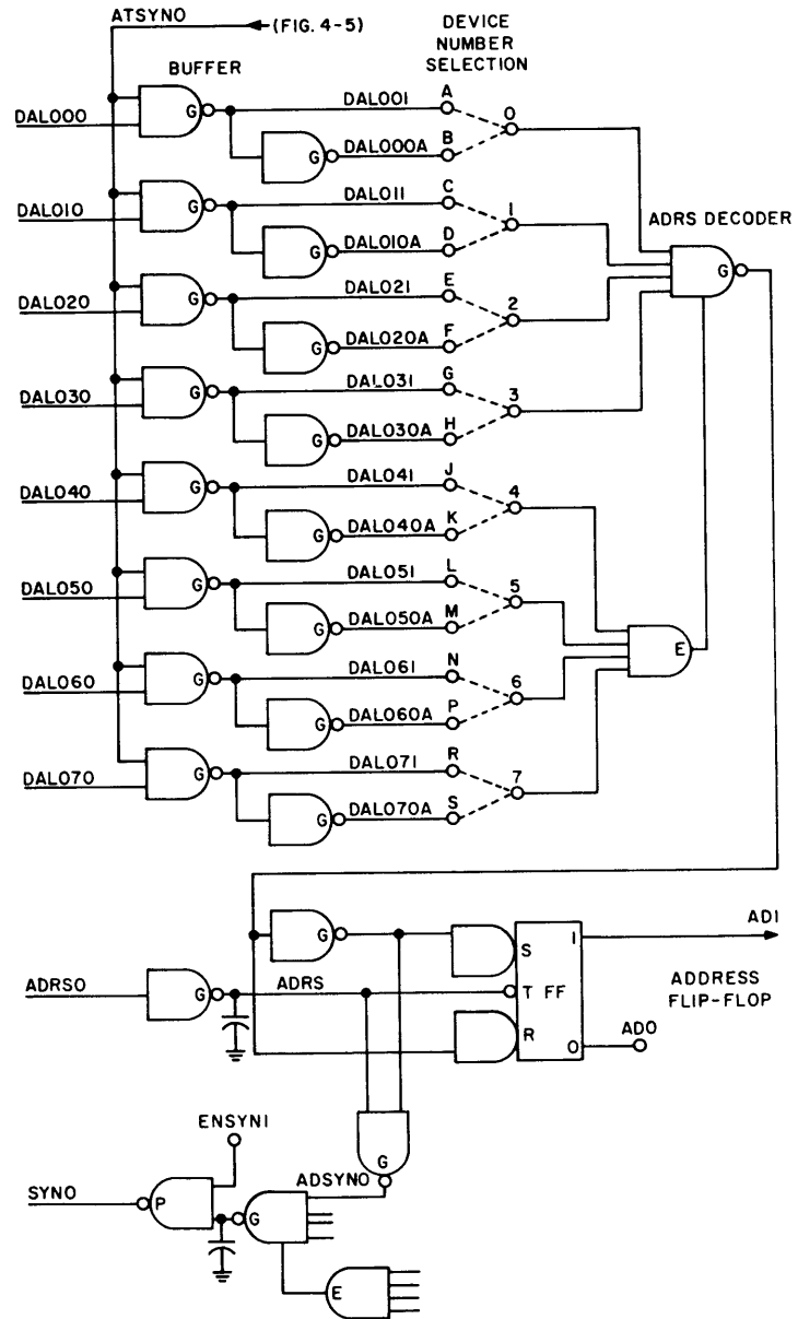
Figure 4-3. Device Addressing, Logic Diagram
