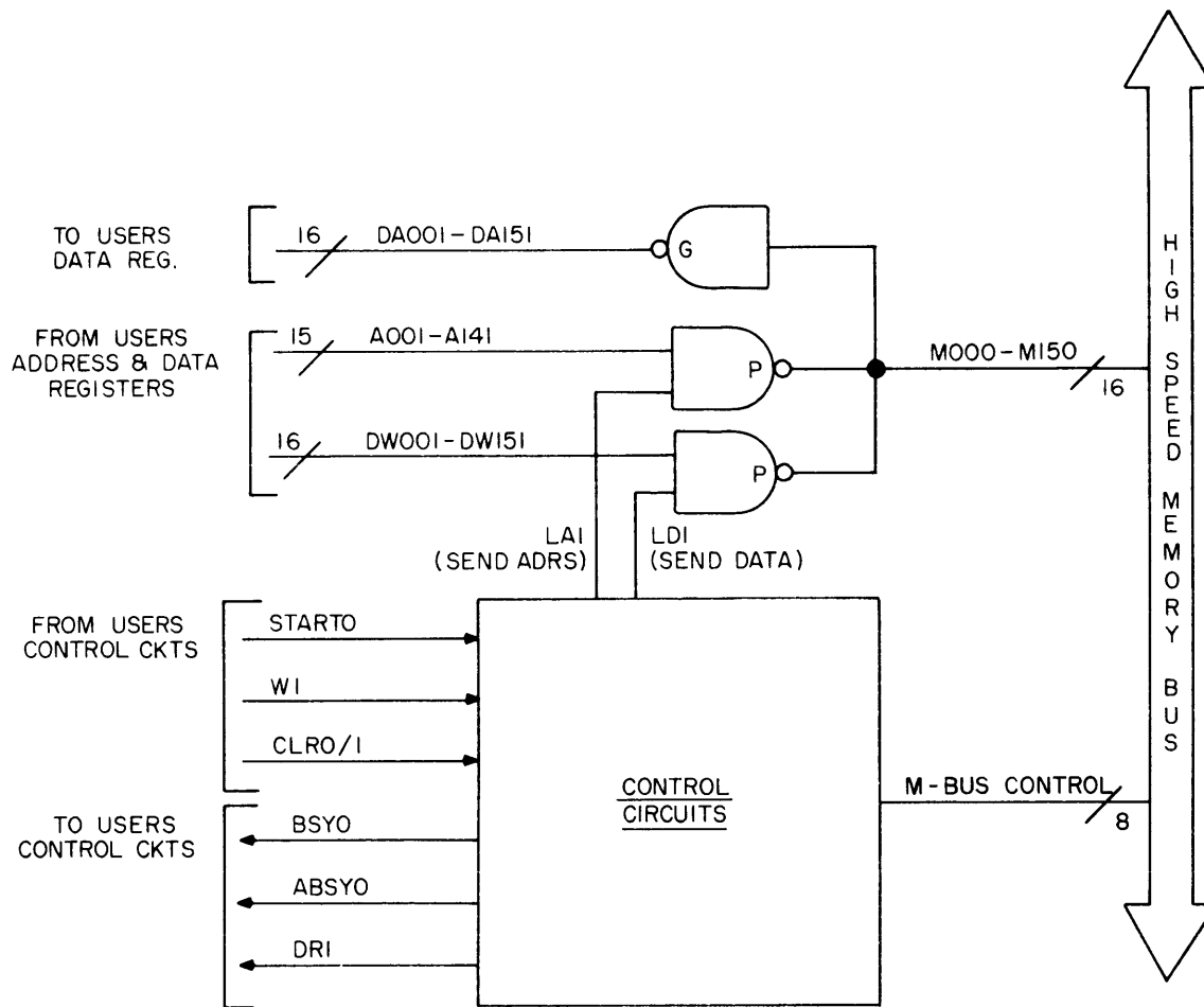
Figure 1-8. SMBI, Block Diagram
