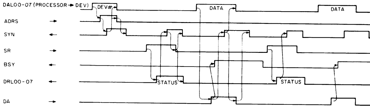
Figure 2-26. Write Block Instruction Timing
