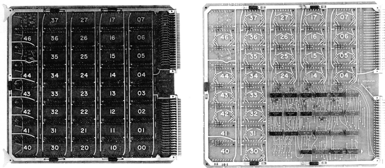
Figure 1-9. Mother-Board Layout
