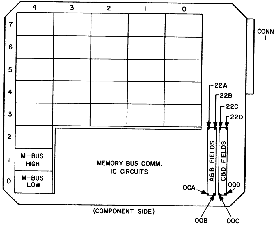
Figure A2-1. SMBI Board Layout
