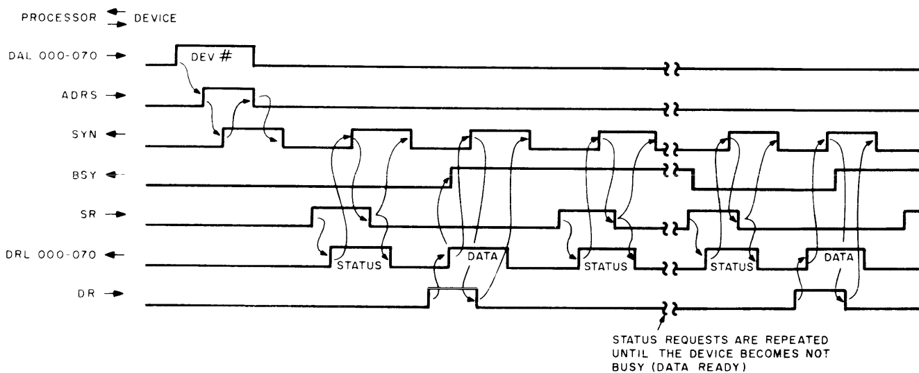
Figure 2-22. Read Block Instruction Timing
