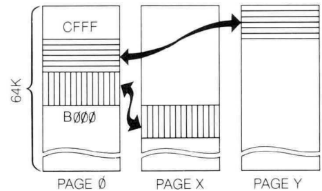
Figure 1. Memory Management in independent mode as usually supplied. Page 0 map is user-selectable to any 4K block.
