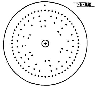
FIGURE 9.2. BCD ENCODER FOR CLOCK
