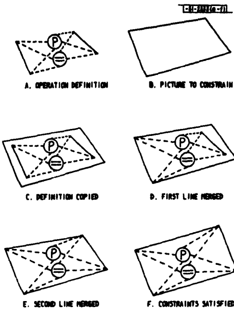
FIGURE 6.1. APPLYING TWO CONSTRAINTS INDIRECTLY TO TWO LINES
