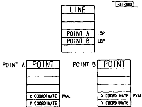
FIGURE 3.1. N-COMPONENT ELEMENTS
