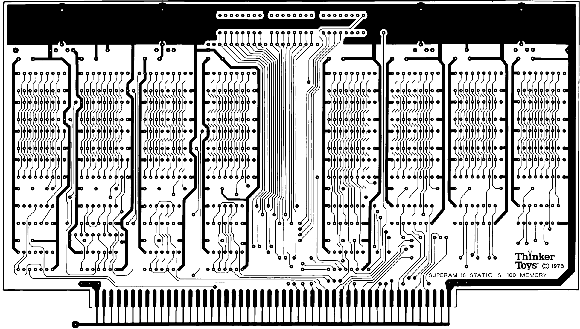
THINKER TOYS SUPERAM 16 STATIC S-100 MEMORY COMPONENT SIDE P.C. DESIGN BY M&M DESIGNS 8-78
