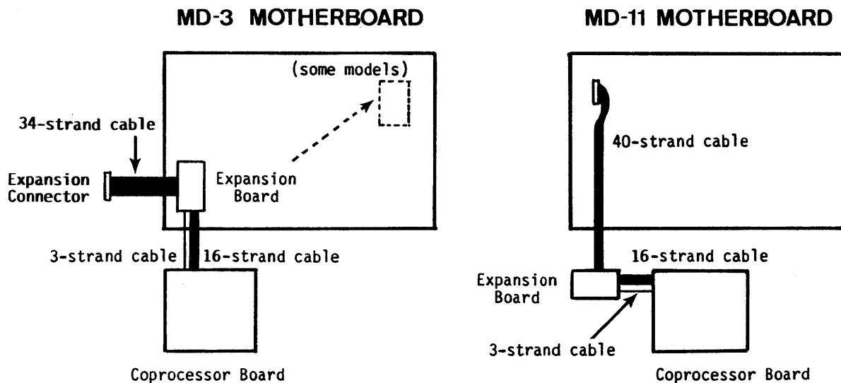
Figure A-1: Hardware Block Diagram
