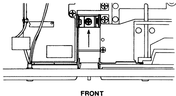
Figure A-5: L-shaped brackets securing drives
