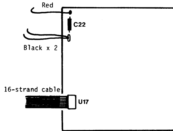
Figure A-17: Installation of cables, Coprocessor Board
