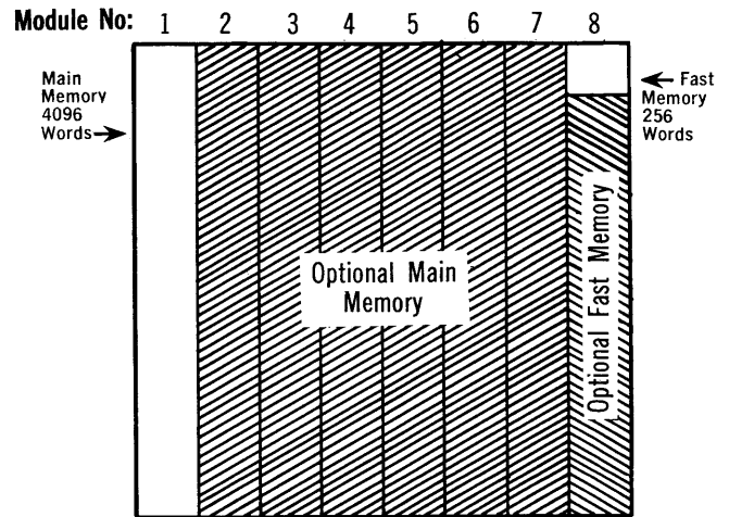
Figure 1. PB440 Overall Memory Layout
