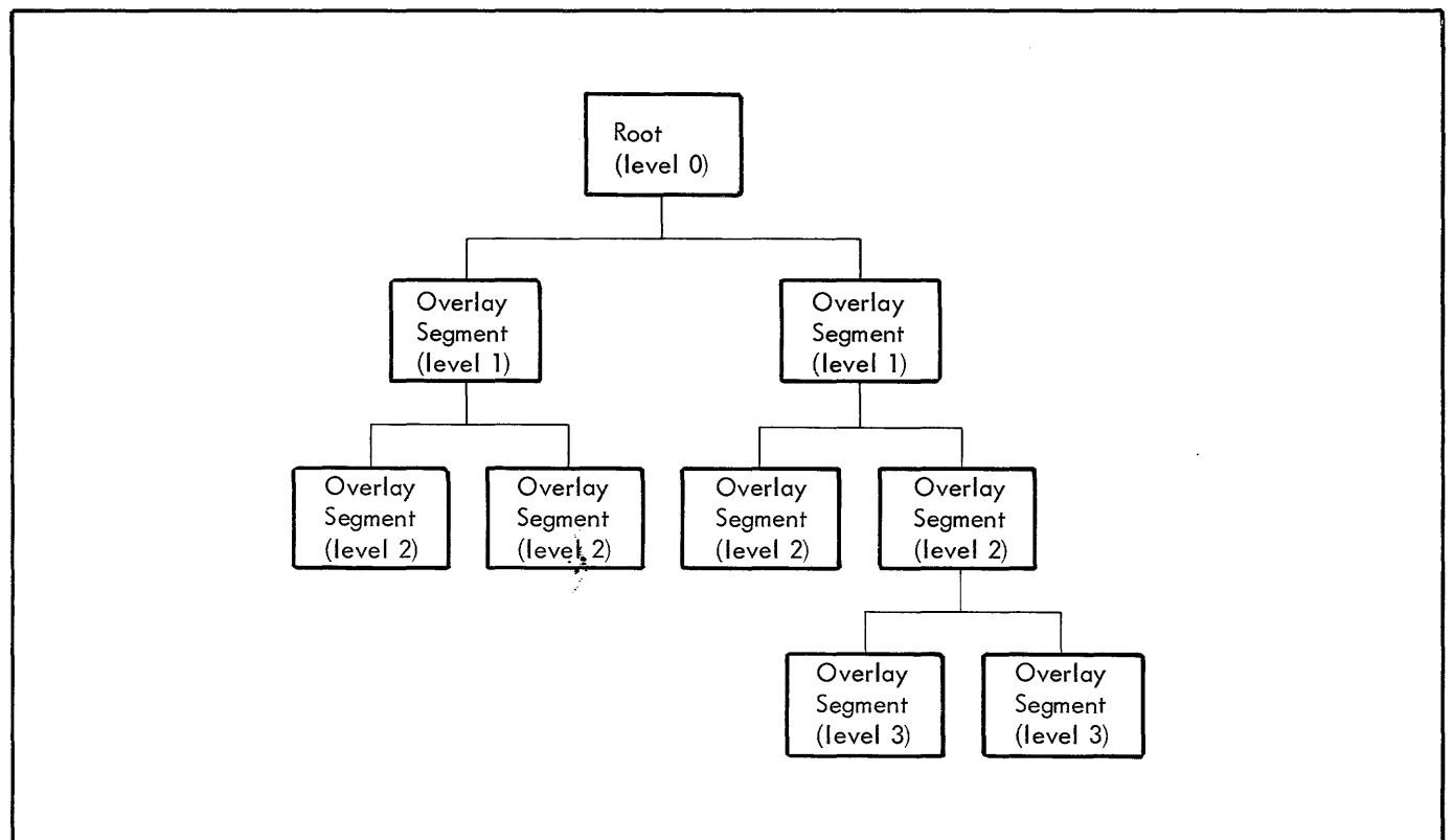
Figure 1. Overlay Structure
