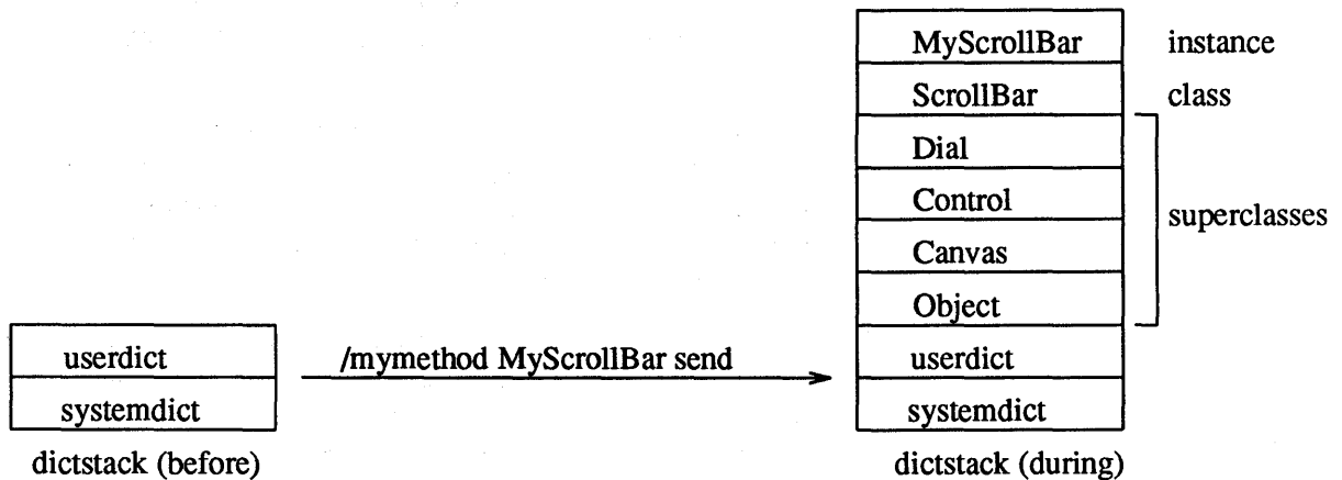
Figure 4-4 Dictionary stack before and during a send to MyScrollBar
