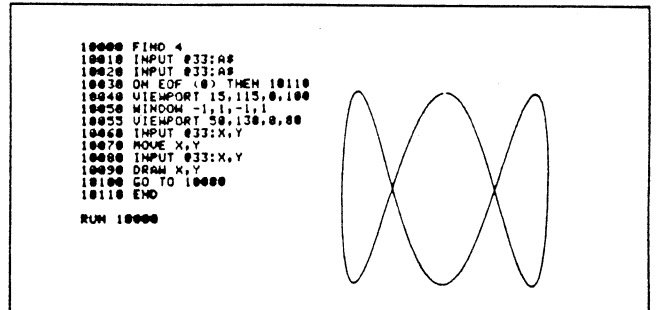
Fig. 7. Program to plot the data in Fig. 6.
