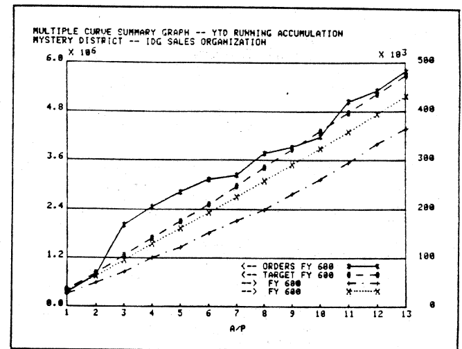
Fig. 2. Since the EXPENSE and BUDGET items were less than 20% of the ORDERS and TARGET items, the program generated a second axis on the right. The arrows in the legend indicate the EXPENSE and BUDGET curves are associated with that axis.
