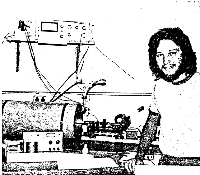
The spinner magnetometer picks up signals as faint as 10^{-7} emu total.
