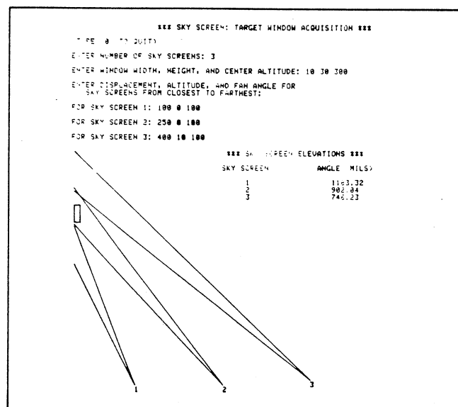
Fig. 10. The Sky Screen closest to the window is angled to view the bottom, the one farthest away to cover the top. Note that three Sky Screens are unnecessary in this case.
