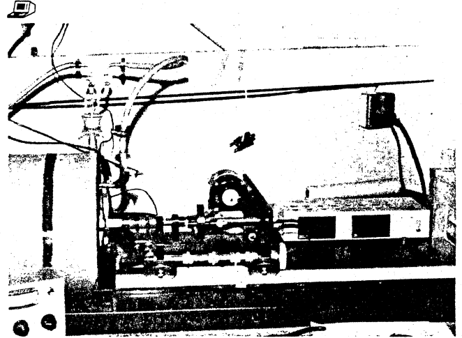
The spinner magnetometer picks up signals as faint as 10^{-7} emu total.
