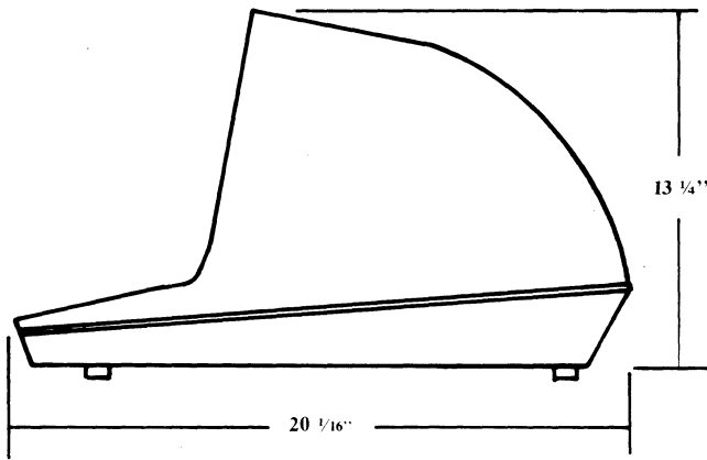
Figure 2-1 Model 910 Dimensions
