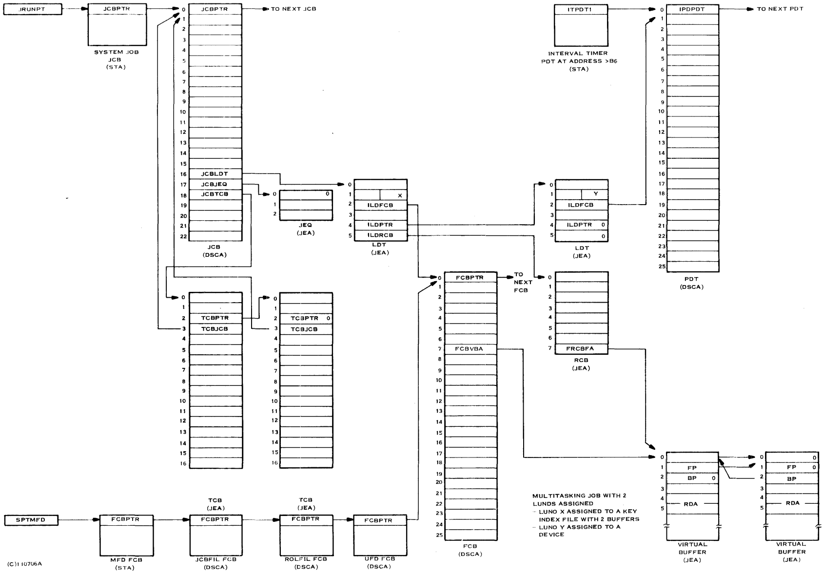
Figure 1. Control Block Linkage
