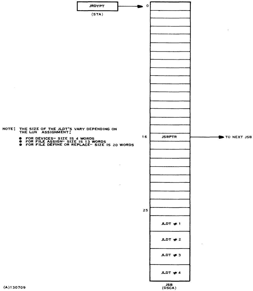
Figure 4. Ready State Job Structure
