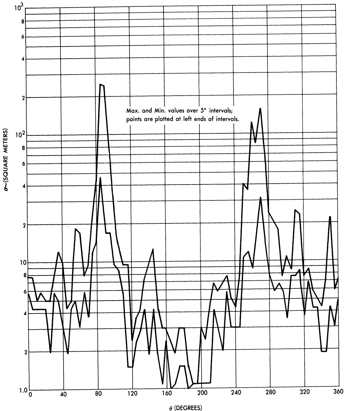
FIG. B-2d CROSS-SECTION OF THE B-47 AIRCRAFT AT 150 MC. - EVANS SIGNAL LABORATORY DATA ( \phi = 45^\circ ; E_\phi )
