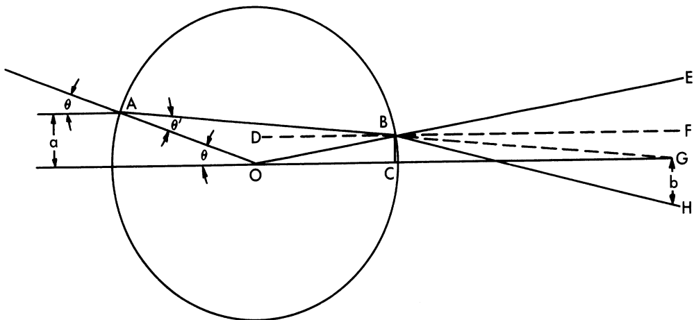
FIG. F-1b SECTIONAL VIEW OF RAY PATHS THROUGH A SPHERICAL LENS
