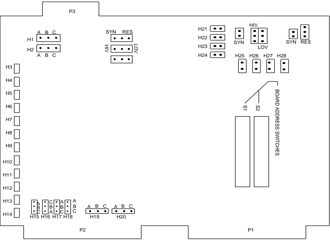
Figure 2-1 Switch and Jumper Locations
